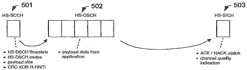
HSDPA frame structure
