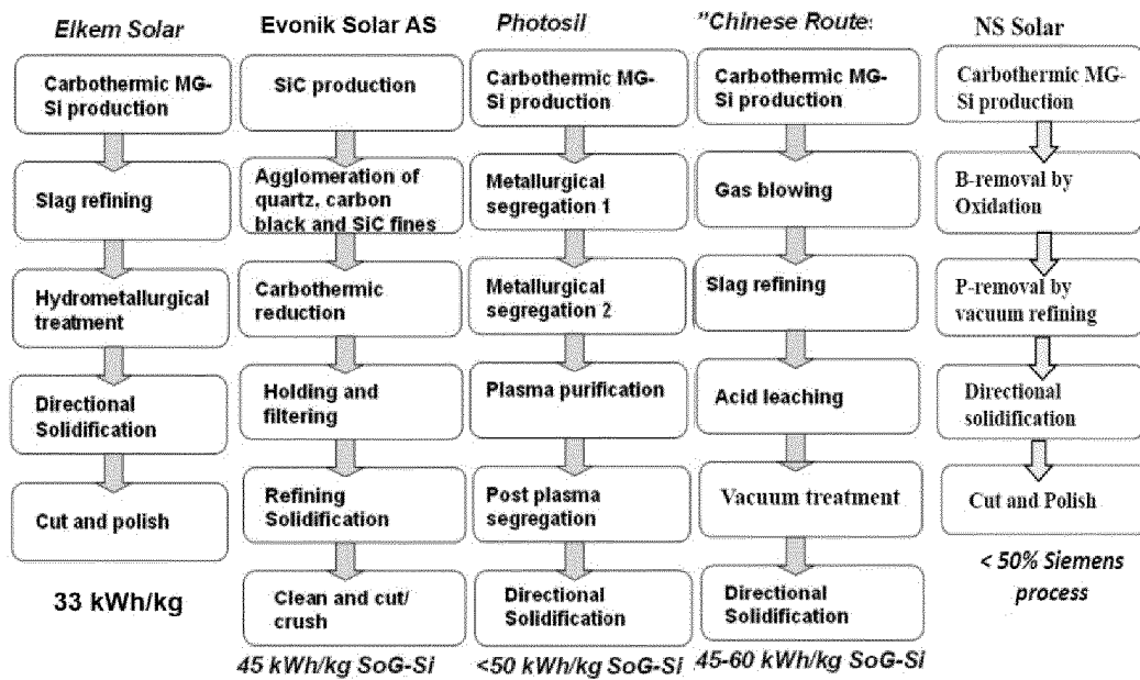
Figure 2: Developed and under development processes for production of SoG-Si.
