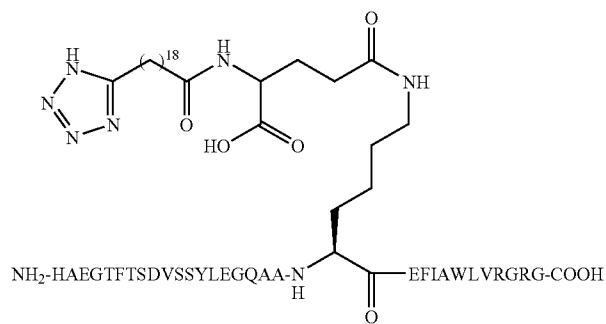
N 26 -(4-(19-(Tetrazol-5-yl)nonadecanoylsulfamoyl)butyryl)[Arg34]GLP-1-(7-37)peptide
