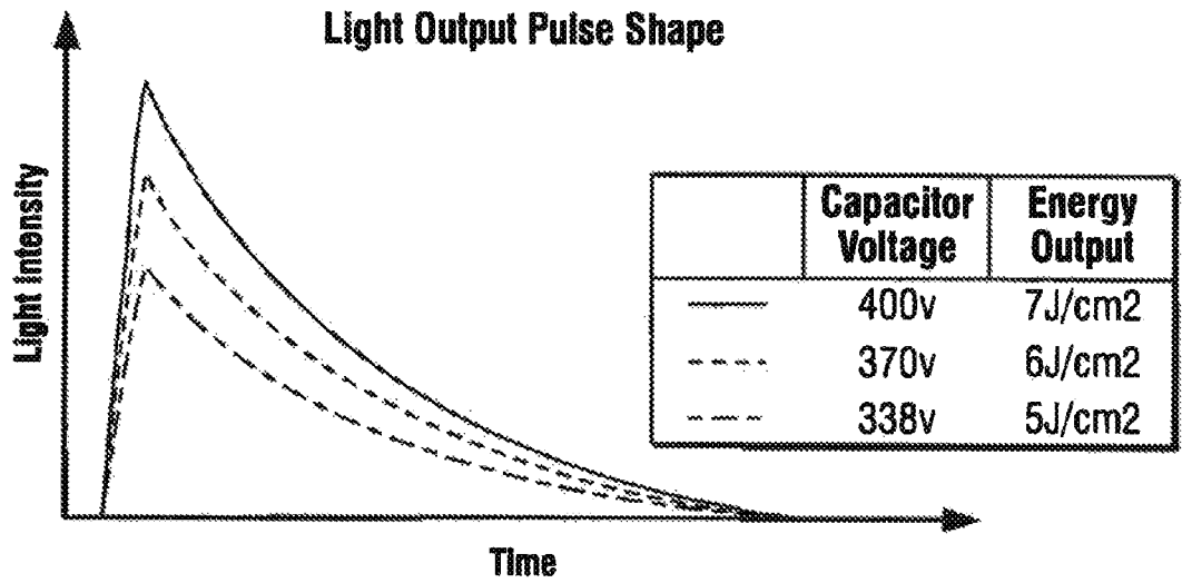
FIG. 1C (PRIOR ART)
