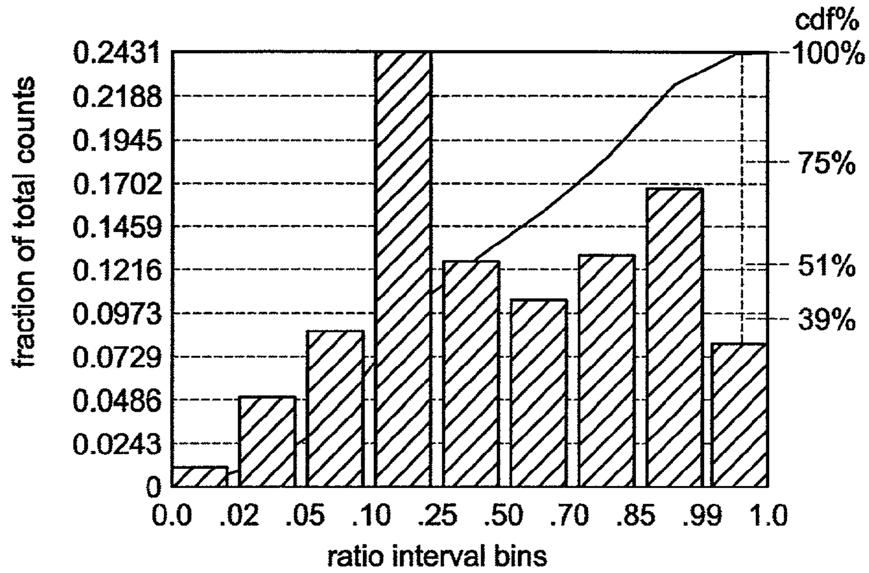
1657 user, program hopping time-watched/time-available
