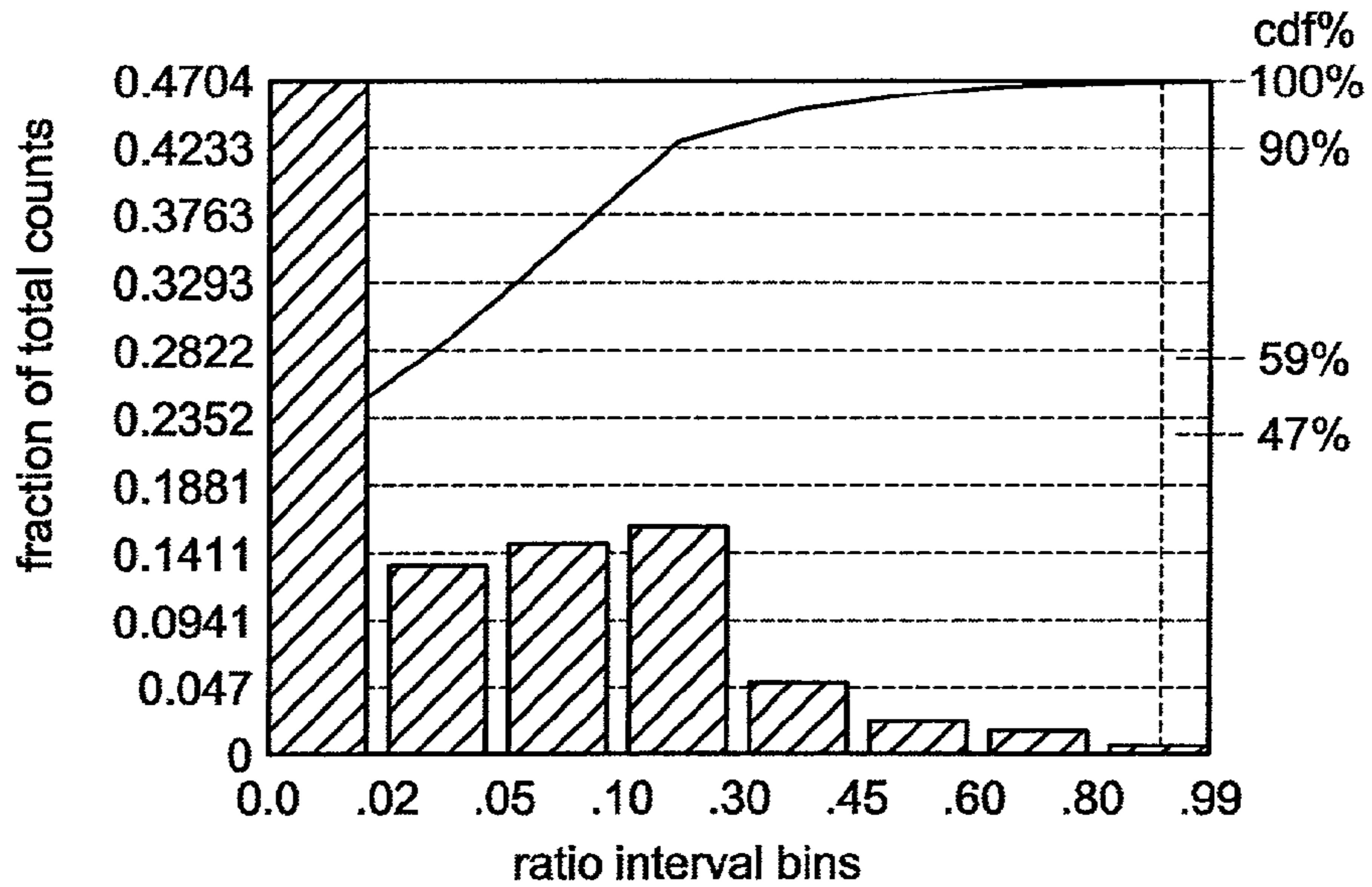
1657 user, time hopped away before returning to program ratio:HopdT/time-avilable
