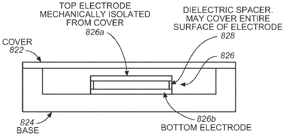
FIG. 8B (SIDE VIEW)
