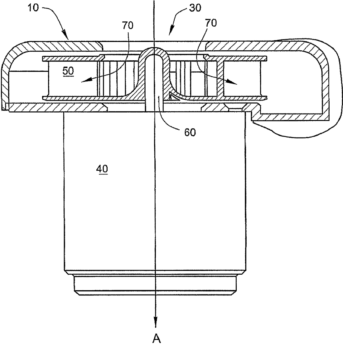
FIG. 2 (PRIOR ART)
