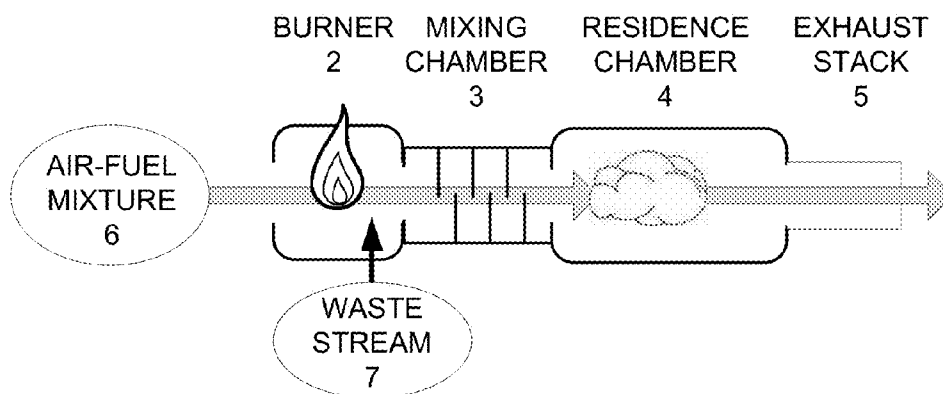
FIG. 1-1A PRIOR ART
