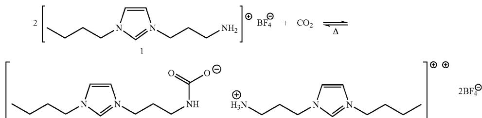
Scheme 2. Proposed reaction between TSIL 1 and CO 2 .
