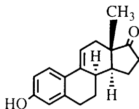
10 \Delta 9(11) -Dehydro-8-isoestrone (VI)
