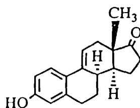
50 \Delta 9(11) -Dehydro-8-isoestron (VI)
