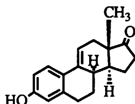
\Delta 9(11)-Dehydro-8-isoestrone (VI)
