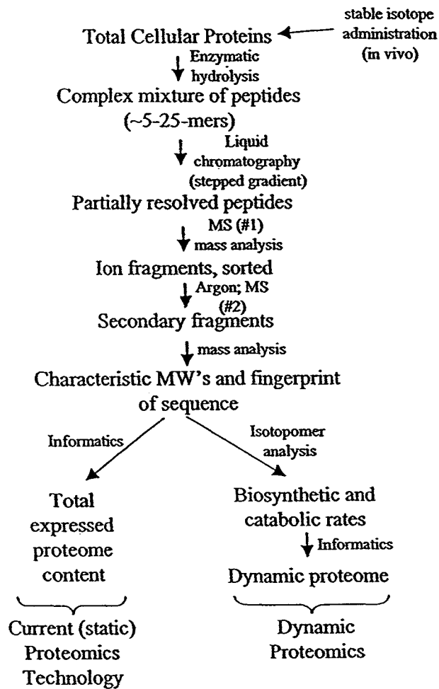
Fig. 3. Technique for Measuring Dynamic Proteomics
