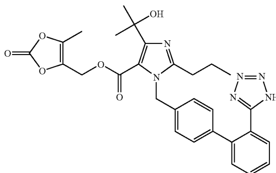
Formula I
