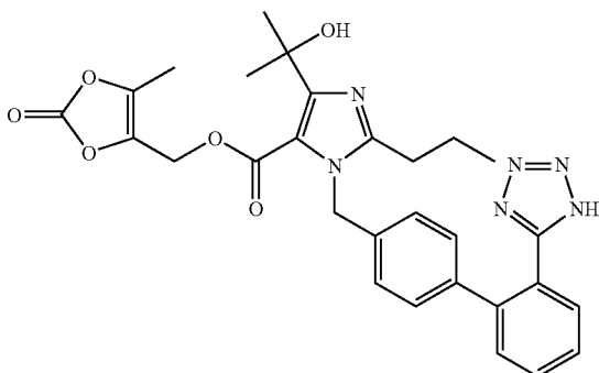
Formula I
