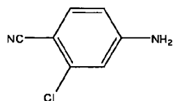
Figure 40. Extracted ion chromatograms (XIC) at m/z 151 of (-) EMS of Compound II incubated in human hepatocytes and proposed chemical structure of the metabolite at m/z 151. The scale of the vertical axis is intensity (CPS). The scale of the horizontal axis is time (minutes).
