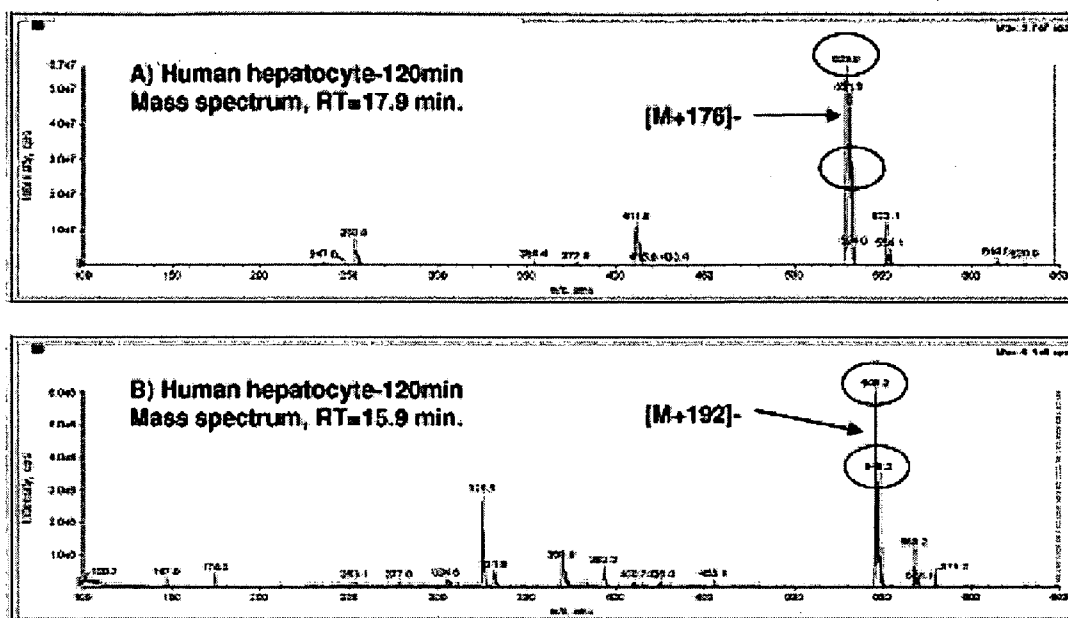
Figure 37. Mass spectra of metabolite(s) of Compound II in human hepatocytes at 17.9 min. The scale of the vertical axis is intensity (CPS). The scale of the horizontal axis is the mass to charge ratio ( m/z ).
