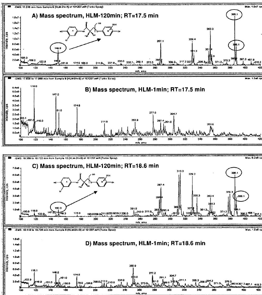
Figure 35. Mass spectra of di-hydroxylated metabolite (negative ion mode, m/z 386) of Compound II at two different retention times (17.5 and 18.6 min) in human liver microsomes. The scale of the vertical axis is intensity (CPS). The scale of the horizontal axis is the mass to charge ratio (m/z).
