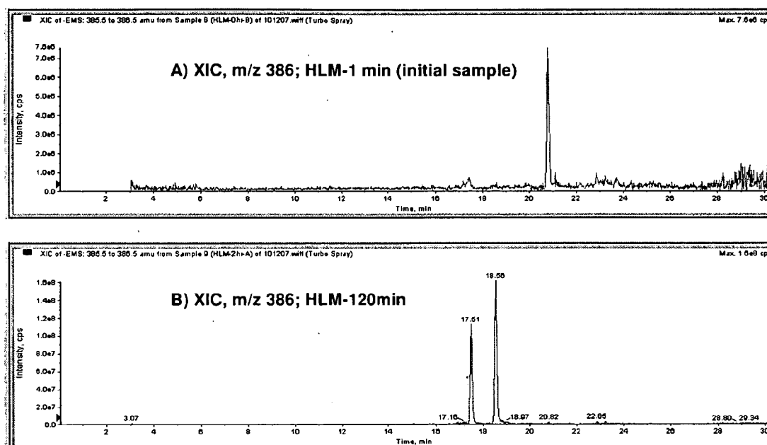
Figure 34. Extracted ion chromatograms (XIC) of di-hydroxylated metabolite (negative ion mode, m/z 386) of Compound II at three different retention times (~17.5 and 18.6 after 120 min, ~20.8 min at initial) in human liver microsomes. The scale of the vertical axis is intensity (CPS). The scale of the horizontal axis is the mass to charge ratio ( m/z ).
