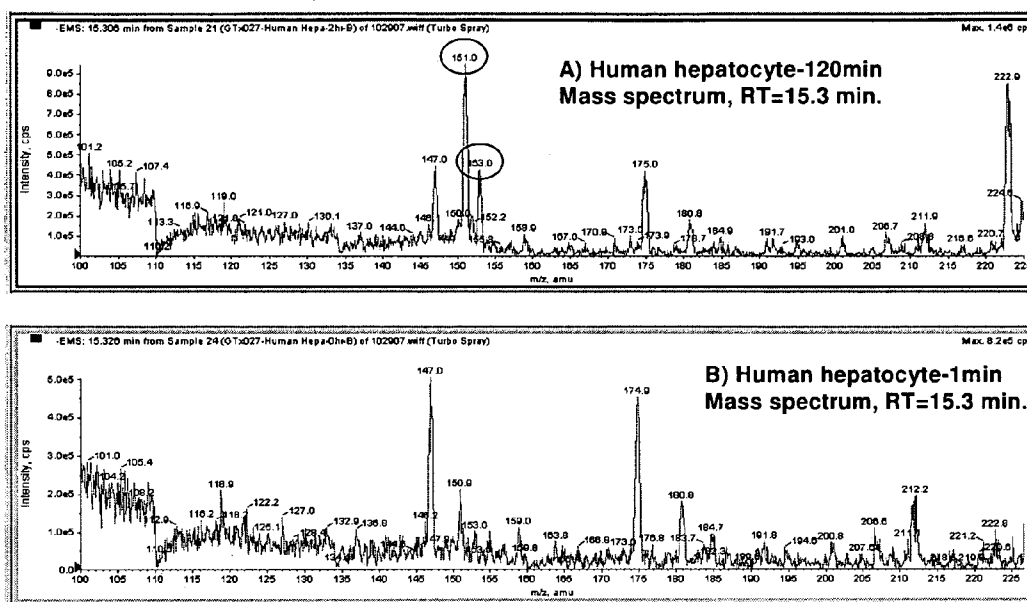
Figure 41. Mass spectra of metabolite of Compound II at m/z 151 in human hepatocytes. The scale of the vertical axis is intensity (CPS). The scale of the horizontal axis is the mass to charge ratio ( m/z ).
