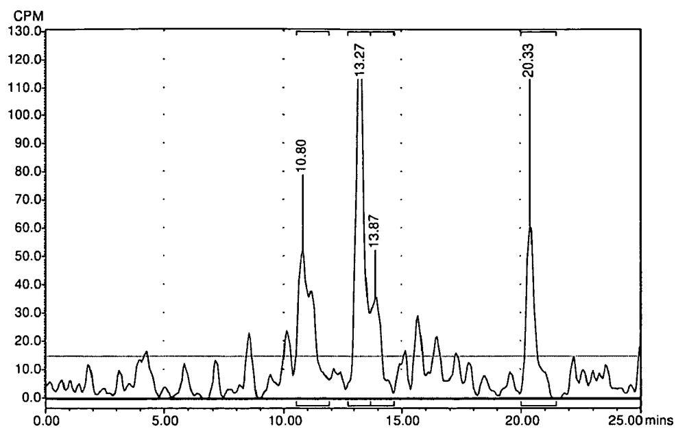
Radiochromatogram of sample from fecal-Pool 3 (BDC Male) following oral administration of Compound I to male Sprague Dawley rats
