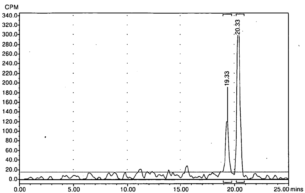
Radiochromatogram of sample from Fecal-Pool 1 (Intact Male) following oral administration of Compound I to male Sprague Dawley rats
