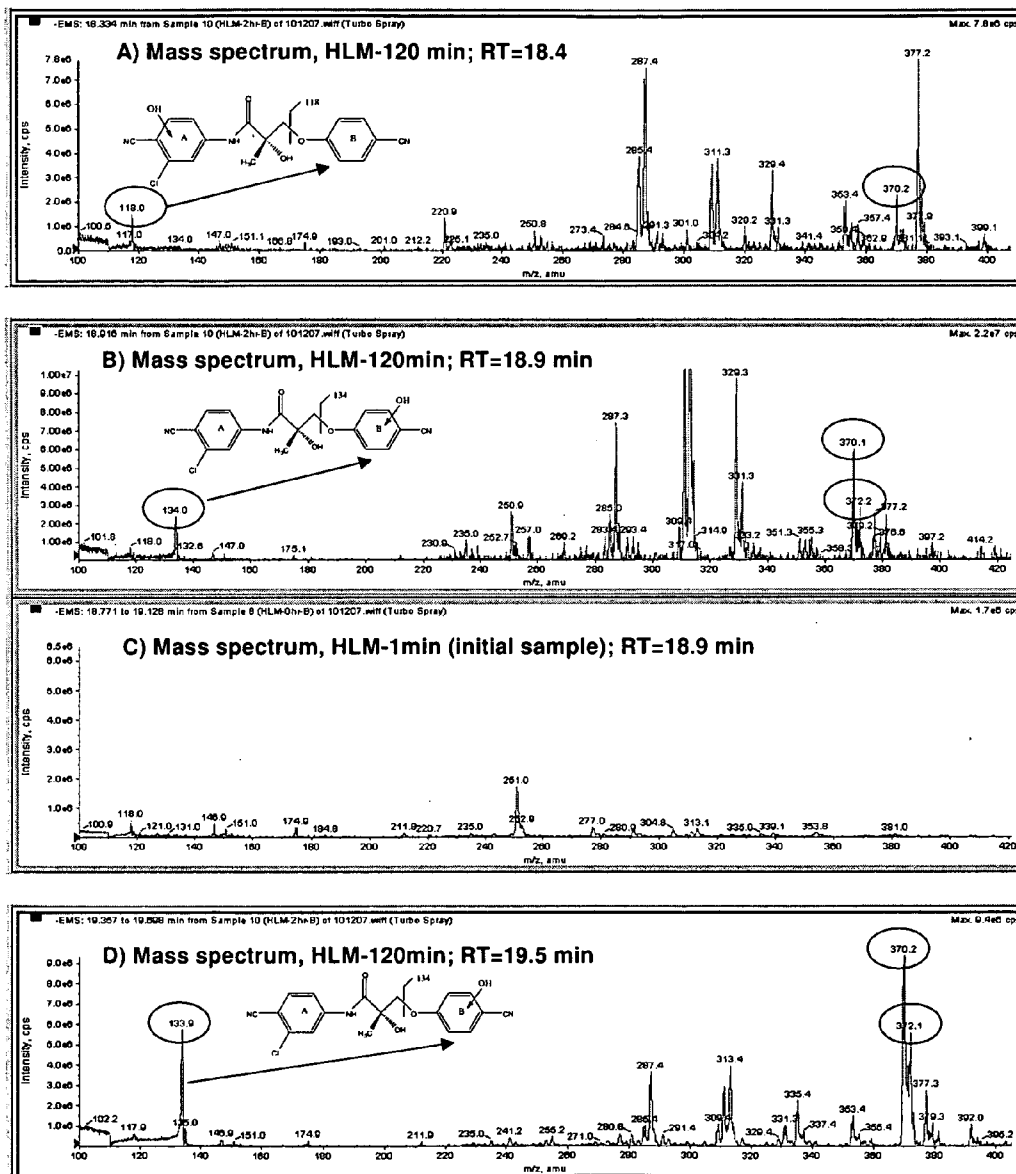
Figure 33. Mass spectra of mono-hydroxylated metabolite (negative ion mode, m/z 370) of Compound II at three different retention times (18.4, 18.9, and 19.5 min) in human liver microsomes. The scale of the vertical axis is intensity (CPS). The scale of the horizontal axis is the mass to charge ratio ( m/z ).
