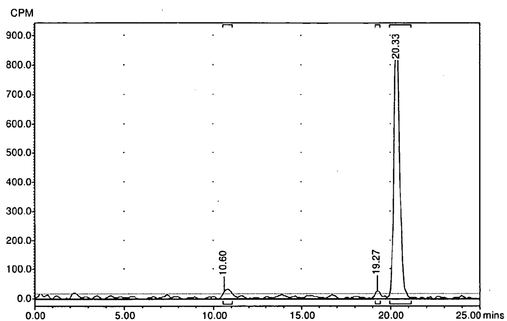
Radiochromatogram of sample from fecal-Pool 2 (Intact Female) following oral administration of Compound I to female Sprague Dawley rats
