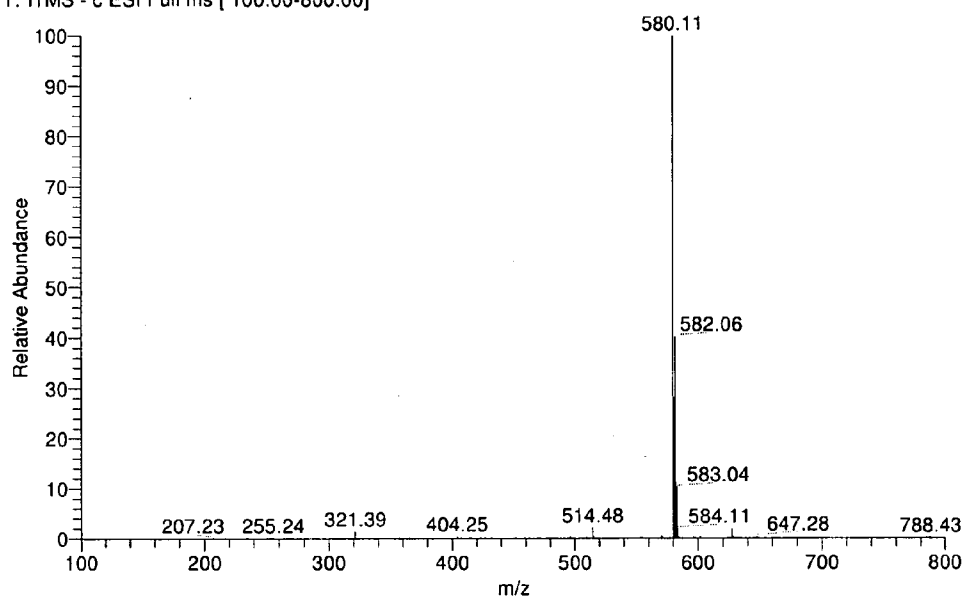
Figure 27. Mass spectrum of the peak at 14.1 min retention time in rat bile showing a molecular ion at m/z 580 for Compound I metabolite II (negative ion mode, [M-H]^- = 580 ). The scale of the vertical axis is relative abundance. The scale of the horizontal axis is the mass to charge ratio ( m/z ).
