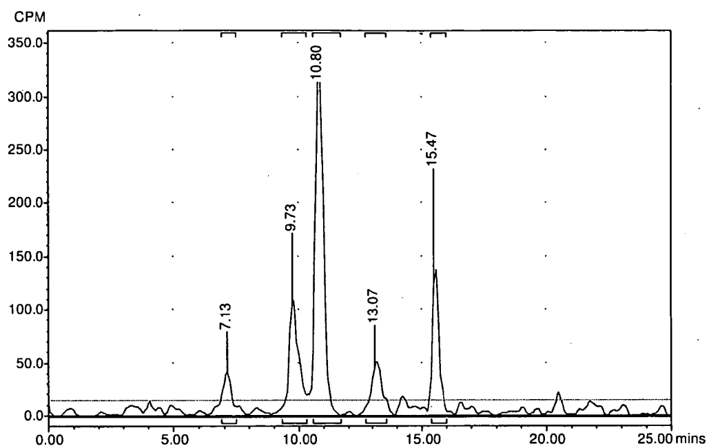
Radiochromatogram of sample from urine-Pool 2 (Intact Female) following oral administration of Compound I to female Sprague Dawley rats
