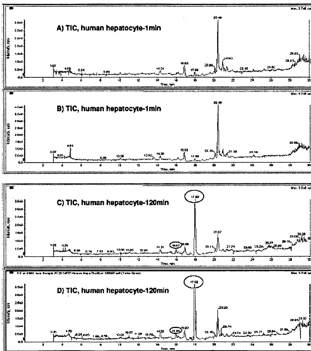
Figure 36. Total ion chromatogram (TIC) of (-) enhanced MS (EMS) of Compound II incubated in human hepatocytes. The scale of the vertical axis is intensity (CPS). The scale of the horizontal axis is time (minutes).
