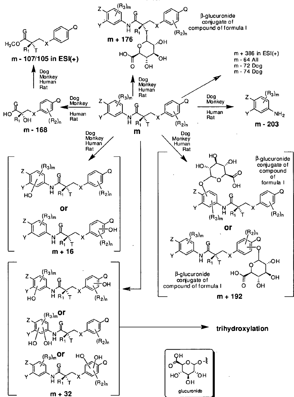
Figure 44. Metabolic map of the general SARM series constructed from in vitro (rat, human, dog, monkey and mouse microsomes and hepatocytes) and in vivo (rat and dog) studies.
