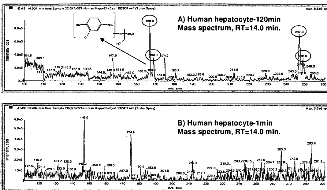
Figure 43. Mass spectra of metabolite of Compound II at m/z 247 in human hepatocytes. The scale of the vertical axis is intensity (CPS). The scale of the horizontal axis is the mass to charge ratio (m/z).
