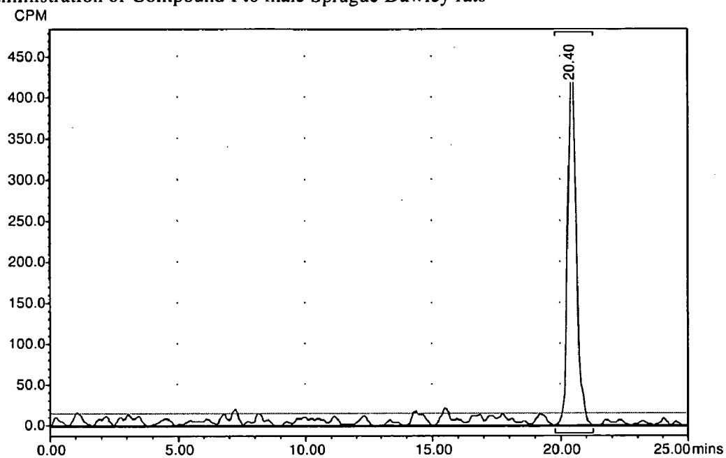
Radiochromatogram of sample from plasma-Pool 1 (JVC Male) following oral administration of Compound I to male Sprague Dawley rats
