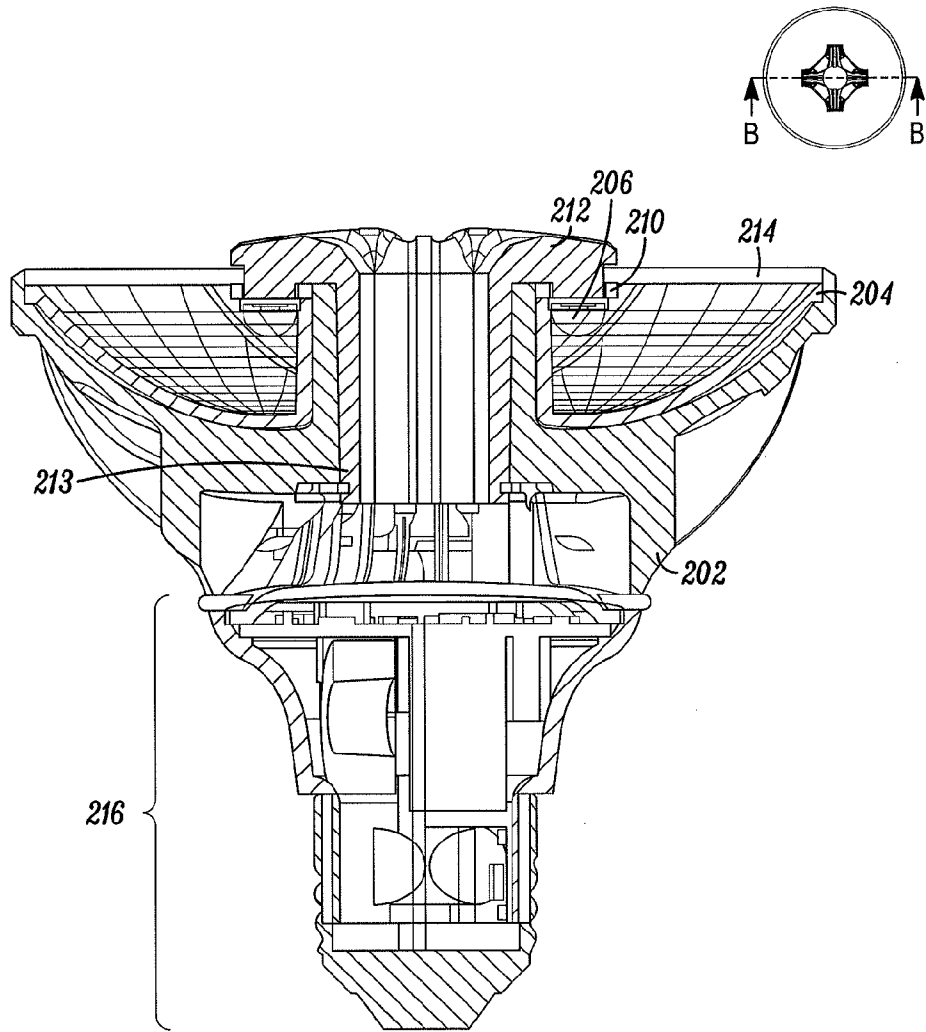
SECTION B-B
