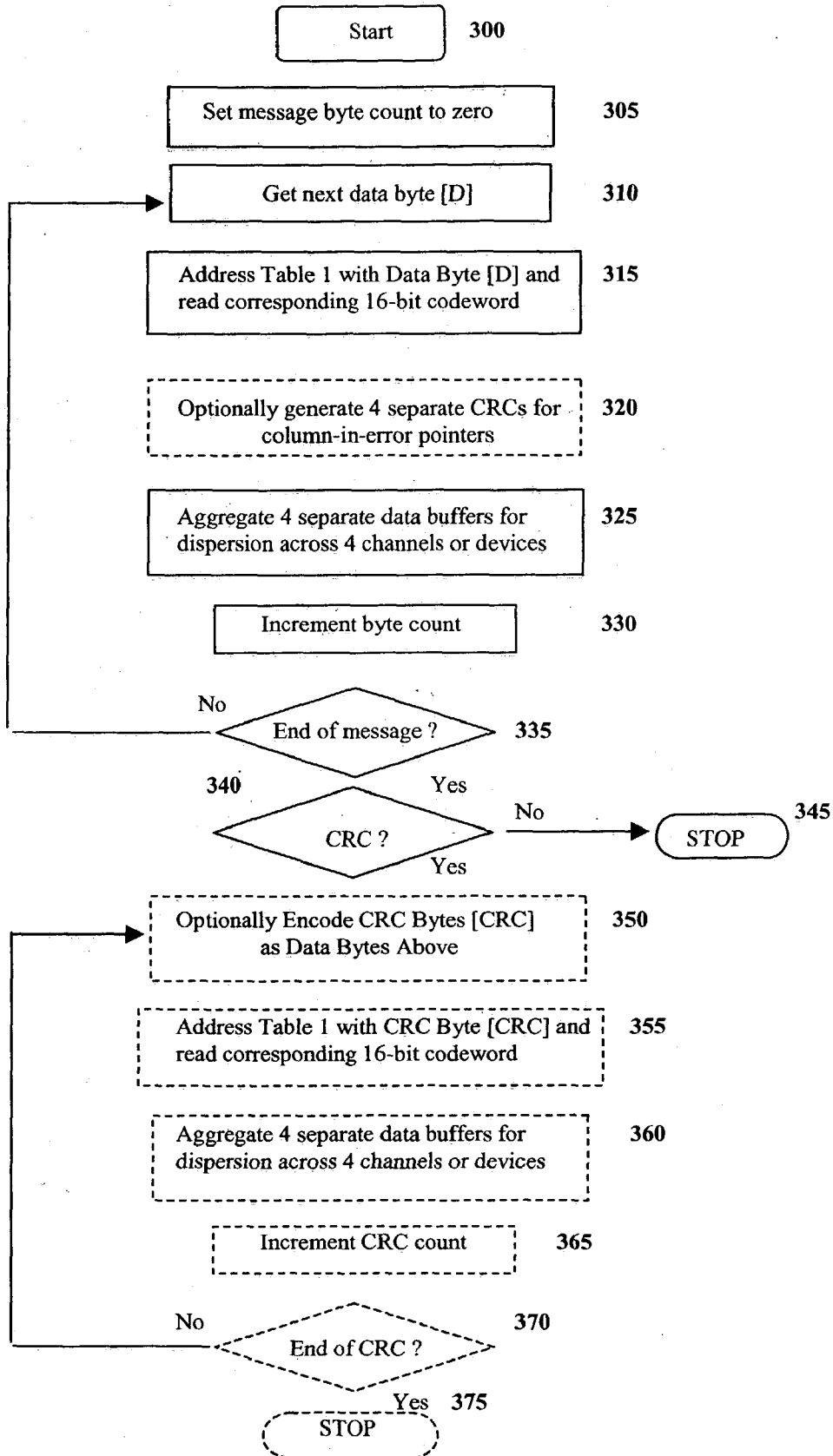
Figure 19 Flowchart for encoding codeword arrays
