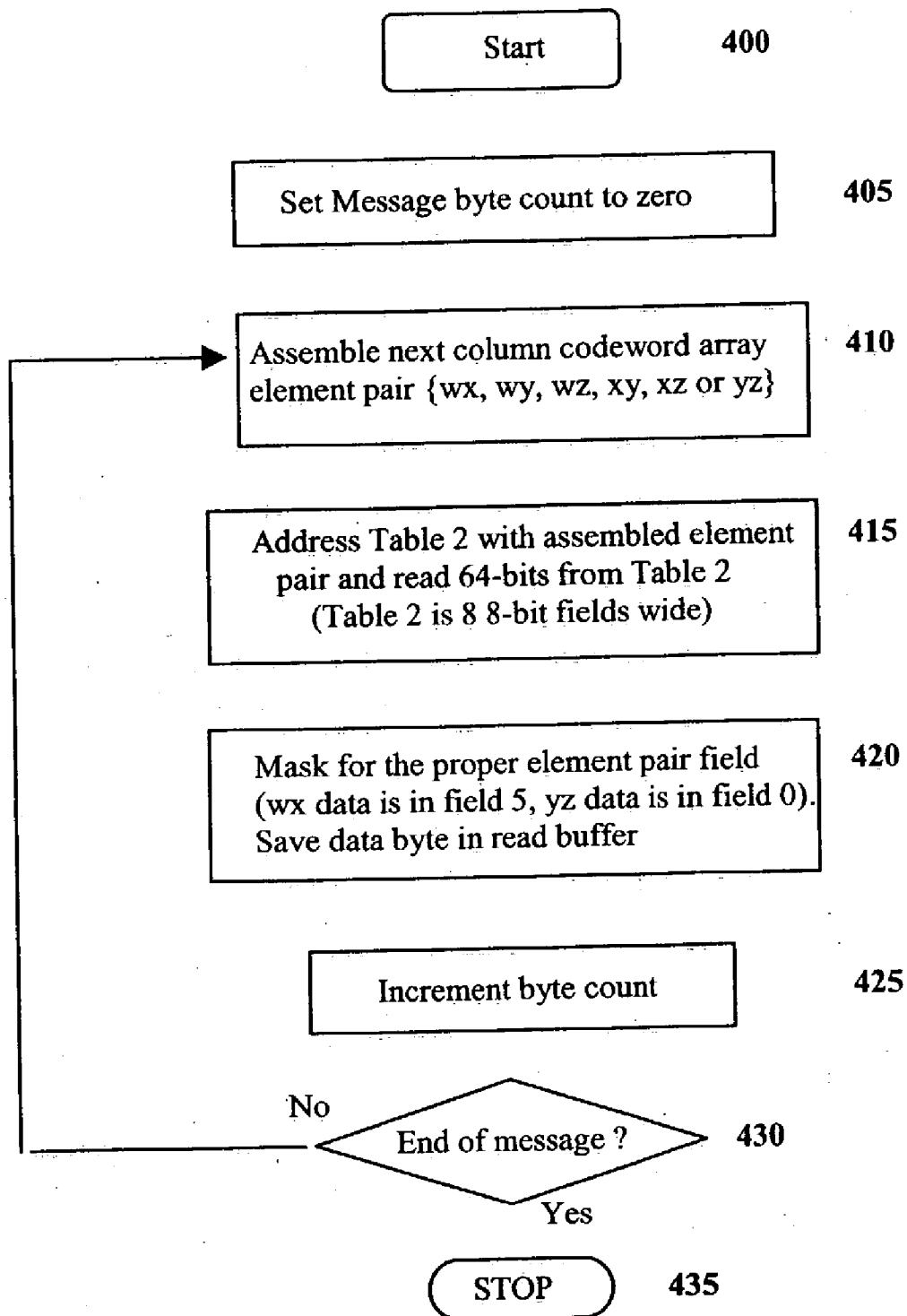
Figure 20 Flowchart for decoding codewords
