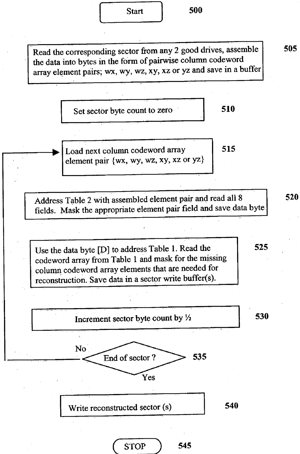
Figure 21 Flowchart for reconstructing a disk drive sector
