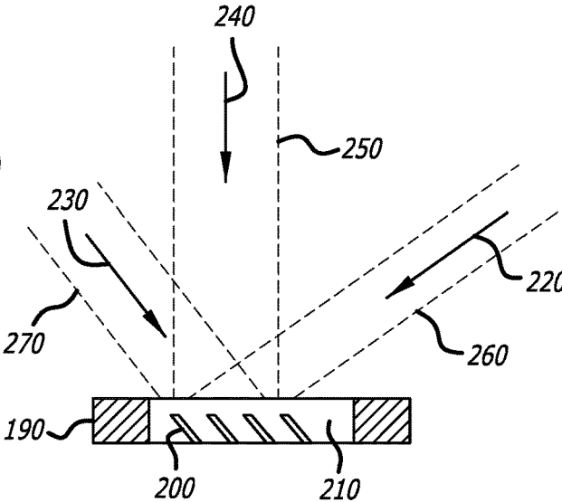
FIG. 3 (Prior Art)
