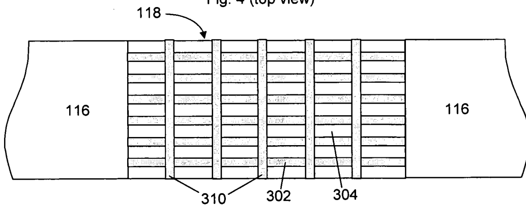
Fig. 4 (top view)
