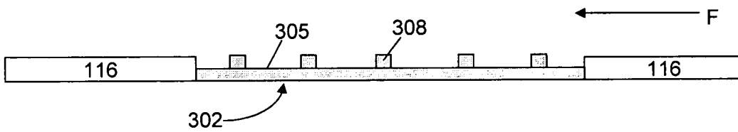
Fig. 3D (end view)
