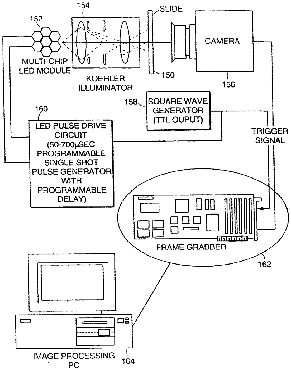
LED KOEHLER ILLUMINATION SYSTEM
