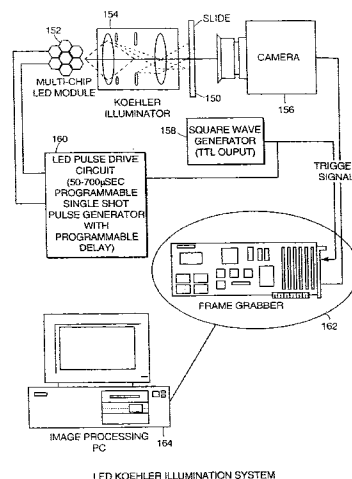
LED KOEHLER ILLUMINATION SYSTEM
