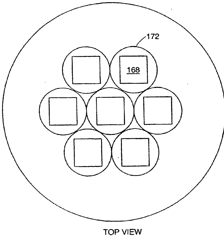
LED MULTICHIP MODULE WITH MICROLENSES
