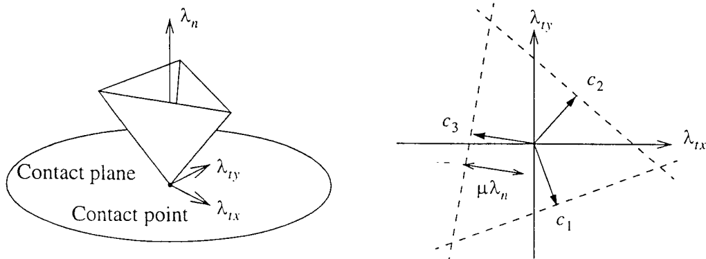
Figure 2.1: The approximated friction cone.
