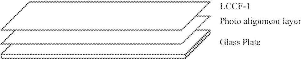
Figure 1: Coating layer stacking of display element of Example 1.
