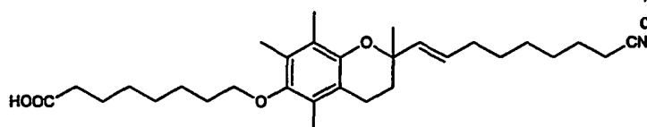
8-[2-(8-Cyano-oct-1-enyl)-2,5,7,8-tetramethyl-chroman-6-yloxy]-octanoic acid
