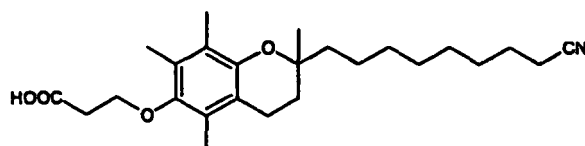
3-[2-(8-Cyano-octyl)-2,5,7,8-tetramethyl-chroman-6-yloxy]-propionic acid
