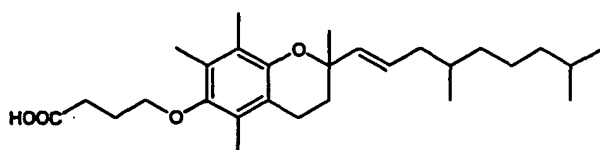
4-[2-(4,8-Dimethyl-nonyl)-2,5,7,8-tetramethyl-chroman-6-yloxy]-butyric acid
