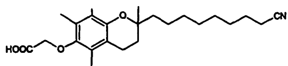
[2-(8-Cyano-octyl)-2,5,7,8-tetramethyl-chroman-6-yloxy]-acetic acid
