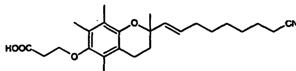
3-[2-(8-Cyano-oct-1-enyl)-2,5,7,8-tetramethyl-chroman-6-yloxy]-propionic acid
