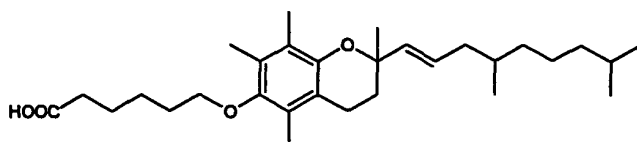
6-[2-(4,8-Dimethyl-nonyl)-2,5,7,8-tetramethyl-chroman-6-yloxy]-hexanoic acid
