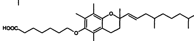
7-[2-(4,8-Dimethyl-nonyl)-2,5,7,8-tetramethyl-chroman-6-yloxy]-heptanoic acid
