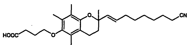
4-[2-(8-Cyano-oct-1-enyl)-2,5,7,8-tetramethyl-chroman-6-yloxy]-butyric acid
