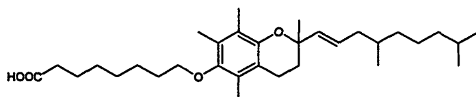
8-[2-(4,8-Dimethyl-nonyl)-2,5,7,8-tetramethyl-chroman-6-yloxy]-octanoic acid
