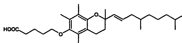
5-[2-(4,8-Dimethyl-nonyl)-2,5,7,8-tetramethyl-chroman-6-yloxy]-pentanoic acid
