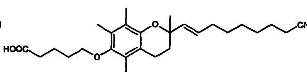
5-[2-(8-Cyano-oct-1-enyl)-2,5,7,8-tetramethyl-chroman-6-yloxy]-pentanoic acid
