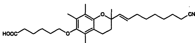
6-[2-(8-Cyano-oct-1-enyl)-2,5,7,8-tetramethyl-chroman-6-yloxy]-hexanoic acid
