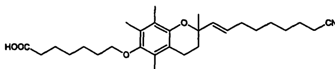
7-[2-(8-Cyano-oct-1-enyl)-2,5,7,8-tetramethyl-chroman-6-yloxy]-heptanoic acid
