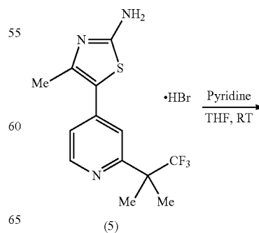
Scheme 3
