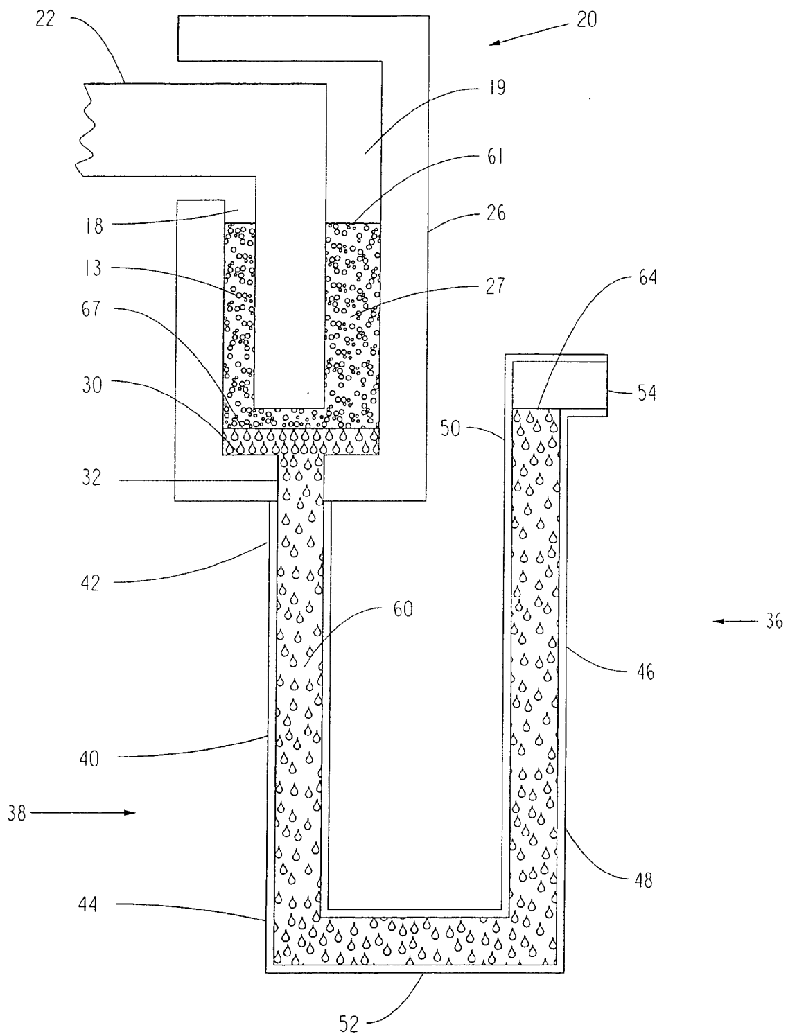
FIGURE 7 PRIOR ART
