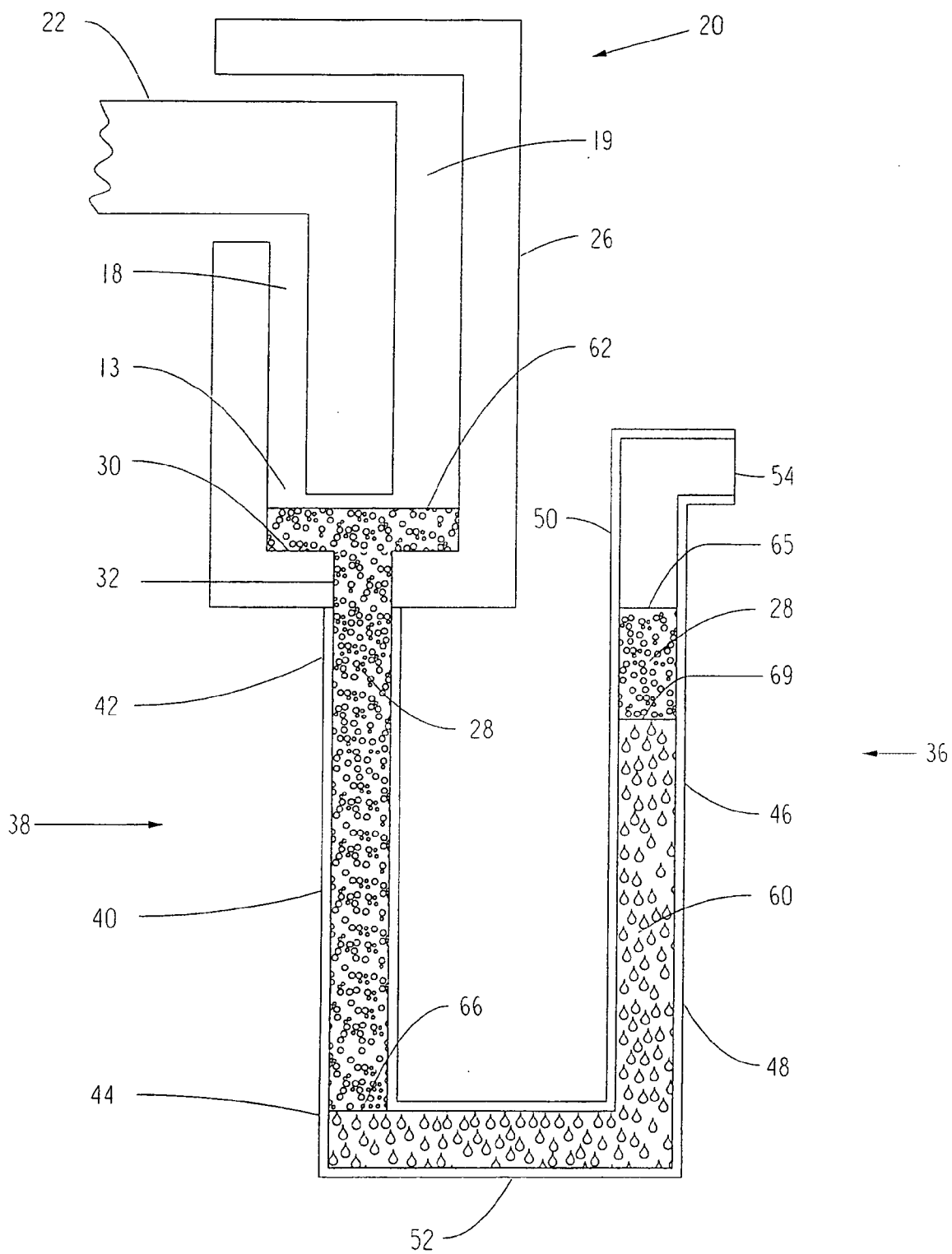
FIGURE 6 PRIOR ART
