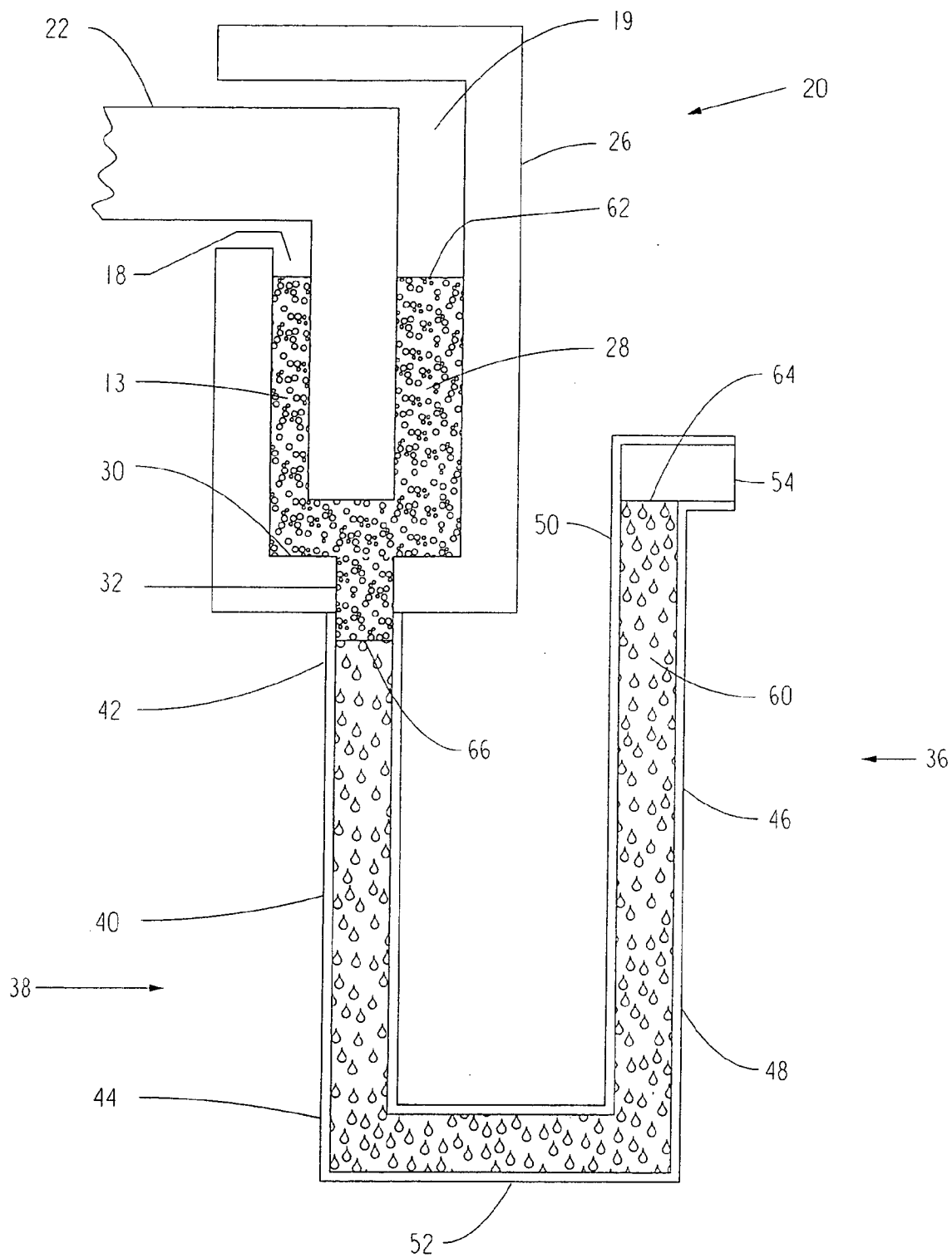
FIGURE 4 PRIOR ART
