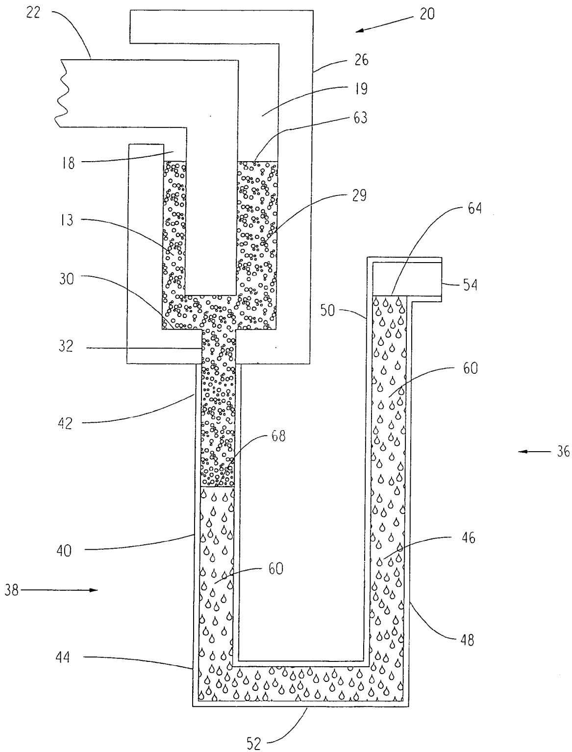
FIGURE 8 PRIOR ART
