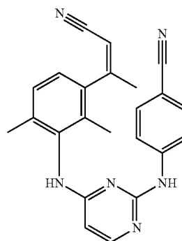
compound 12 = (E) compound 13 = (Z)
