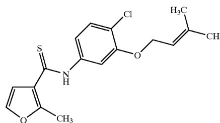
Structure of UC781 TM
