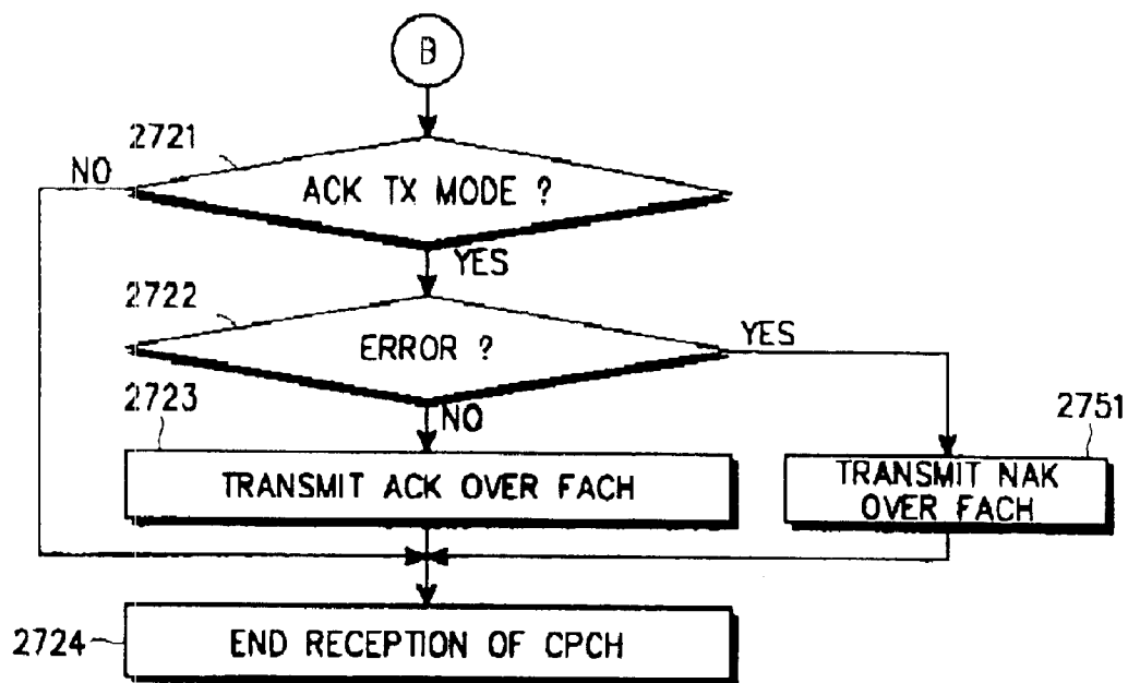
FLOWCHART OF CPCH USING CHANNEL ASSIGNMENT (UTRAN SIDE)
