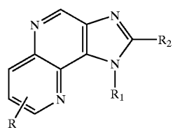
Intermediate Compound 2
