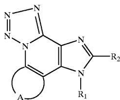
Intermediate Compound 1
