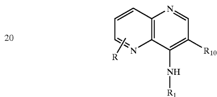
Intermediate Compound 6
