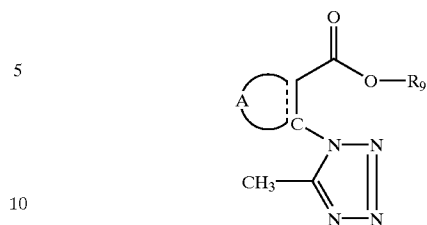
Intermediate Compound 5
