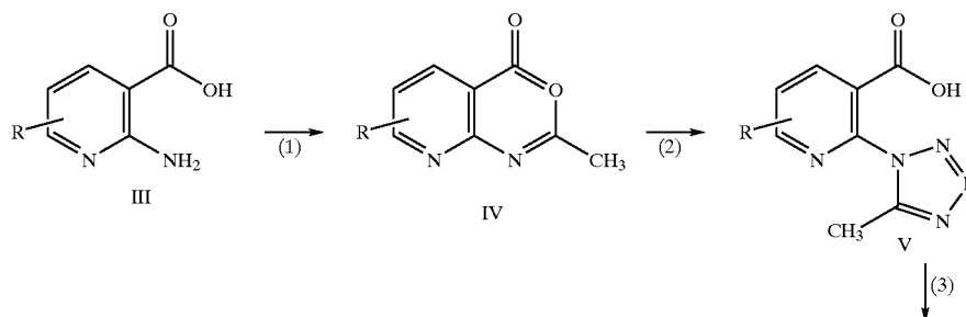
Reaction Scheme I
