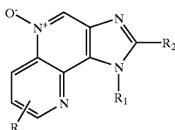
Intermediate Compound 3
