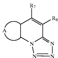
Intermediate Compound 4
