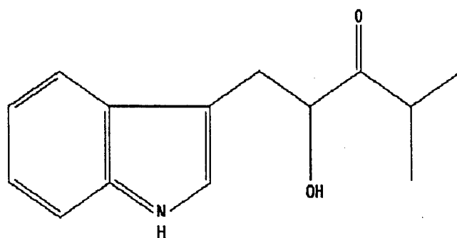
ID4: 3-[2'-hydroxy-4'-methyl-3'-oxopentyl]-indole
