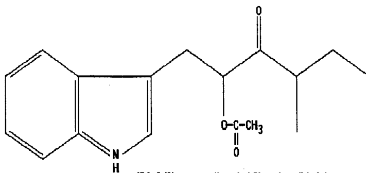
ID1: 3-[2'-acetoxy-4'-methyl-3'-oxohexyl]-indole
