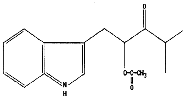
ID2: 3-[2'-acetoxy-4'-methyl-3'-oxopentyl]-indole
