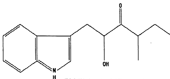
ID3: 3-[2'-hydroxy-4'-methyl-3'-oxohexyl]-indole
