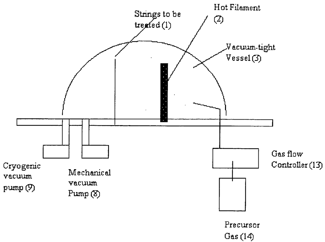
FIG 5: HOT FILAMENT CHEMICAL VAPOR DEPOSITION SYSTEM
