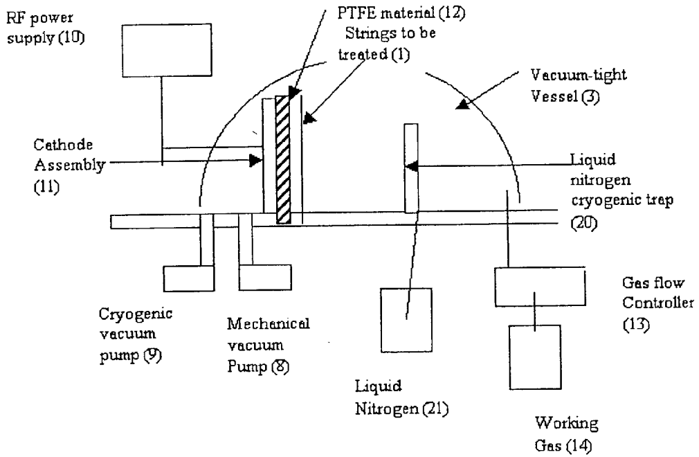
FIG 1: PLASMA SPUTTER DEPOSITION SYSTEM
