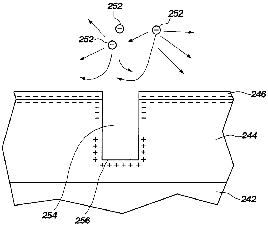
Fig. 8 (PRIOR ART)
