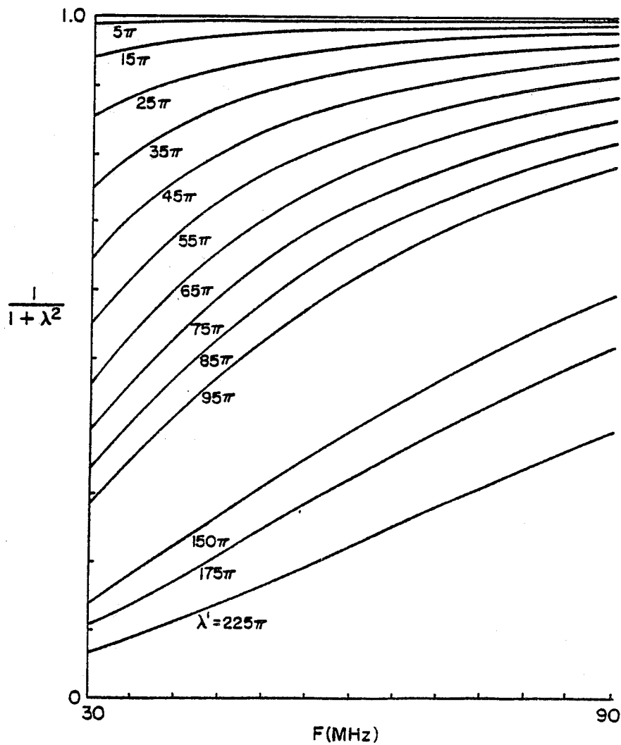
FIG. 2 SERIES RESISTANCE (R-L NETWORK)
