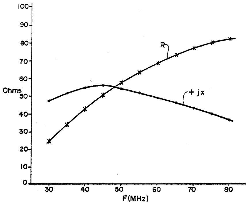
FIG. 9 MEASURED IMPEDANCE vs FREQUENCY
