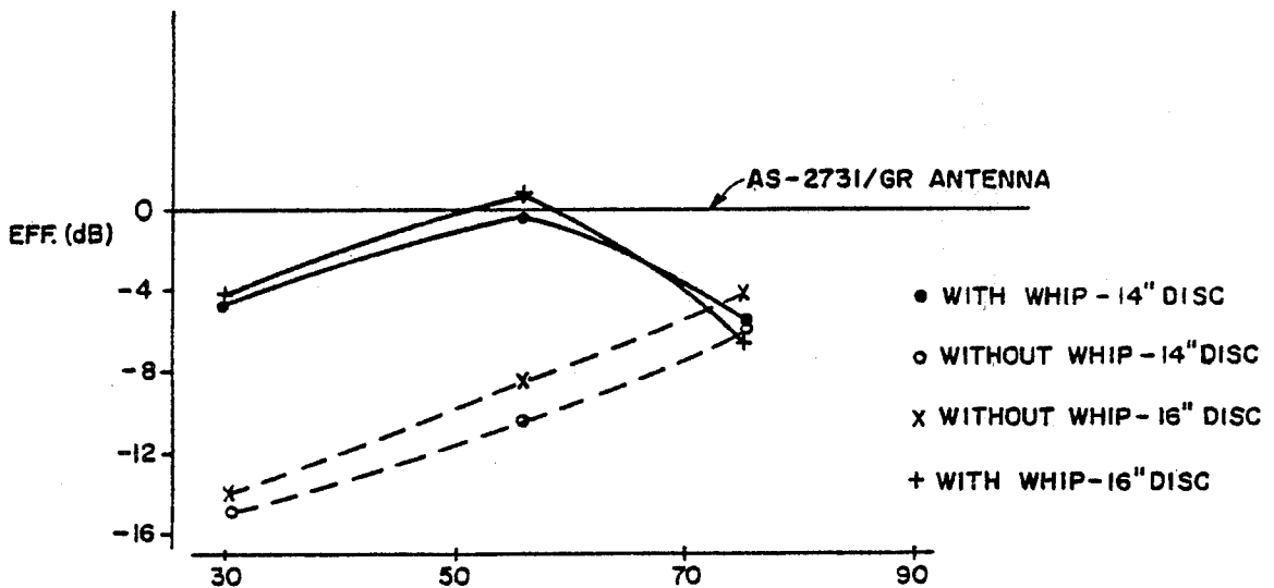
FIG. 16 EFFICIENCY OF SURVIVABLE, LOW PROFILE, ARMOR ANTENNA.
