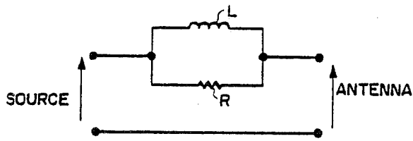
FIG. 1a PARALLEL R/L CIRCUIT, IN SERIES
