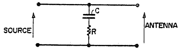
FIG. 1b SERIES R/C CIRCUIT, IN PARALLEL
