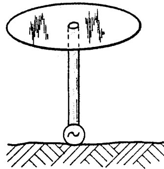
FIG. 5 TOP-LOADED, BASE-DRIVEN ANTENNA
