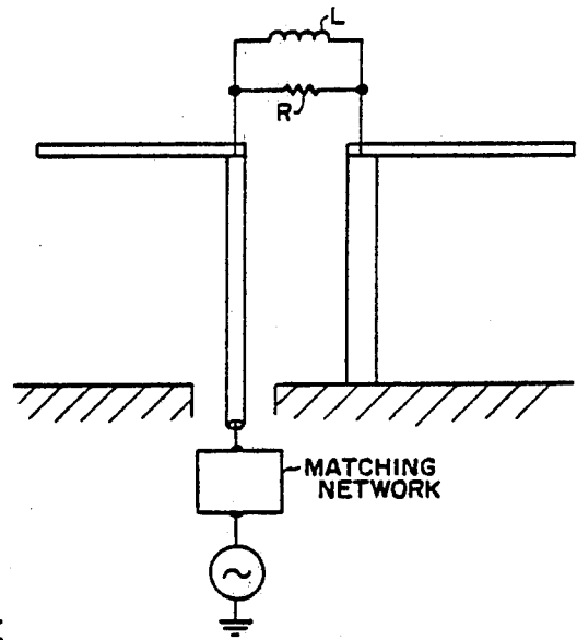
FIG. 15 FOLDED ANTENNA, DISC TOP AND R/L LOADED.
