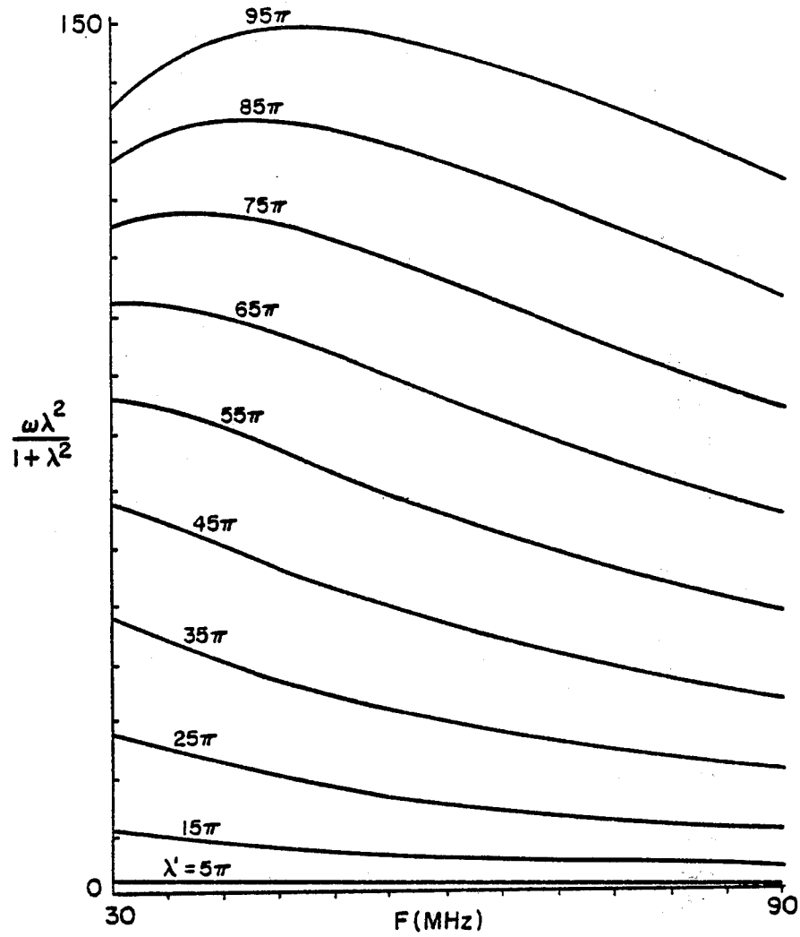
FIG. 3 SERIES REACTANCE, R/L NETWORK
