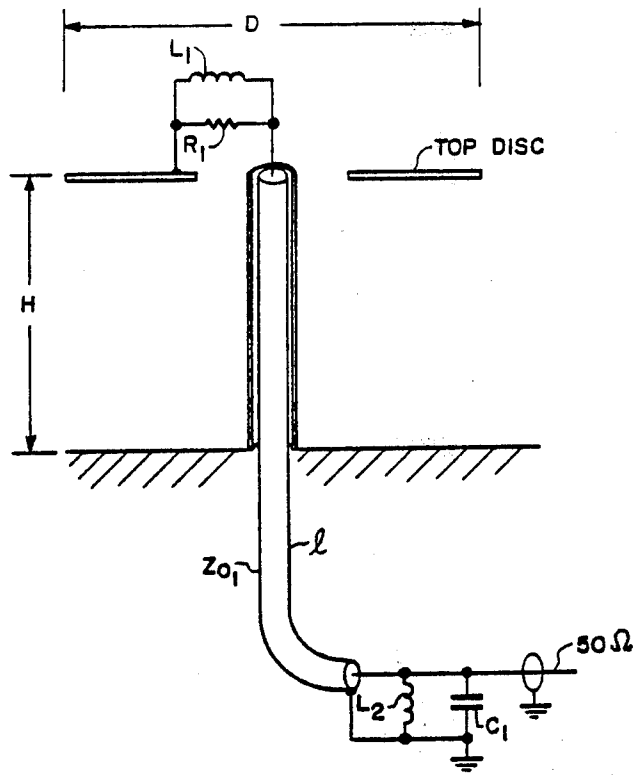
FIG. 11 GROUND BASE TOP-LOADED MONOPOLE
