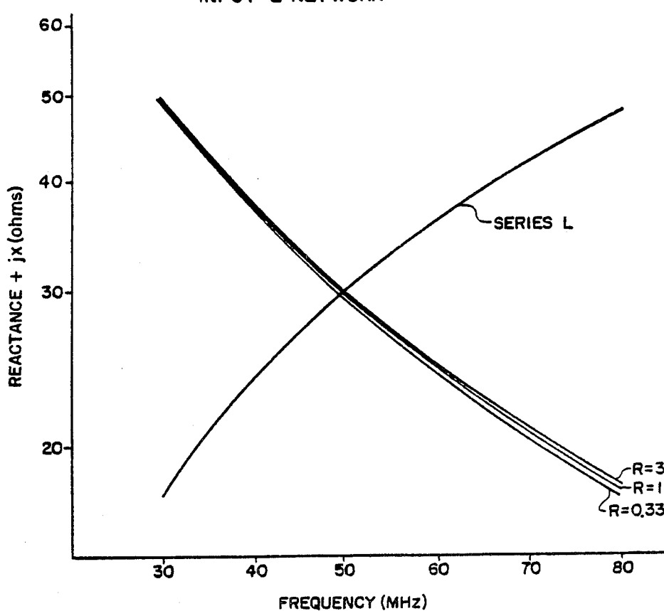
FIG. 8 REACTANCE OF SERIES INPUT L-NETWORK
