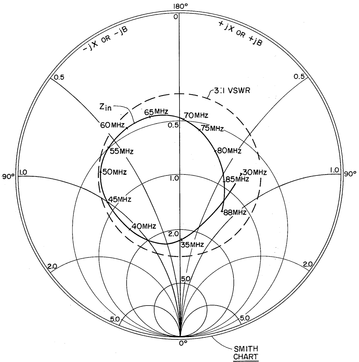
FIG. 7 INPUT IMPEDANCE OF MATCHED ANTENNA AT VHF.
