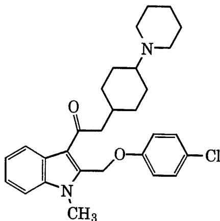
Isomer 2
