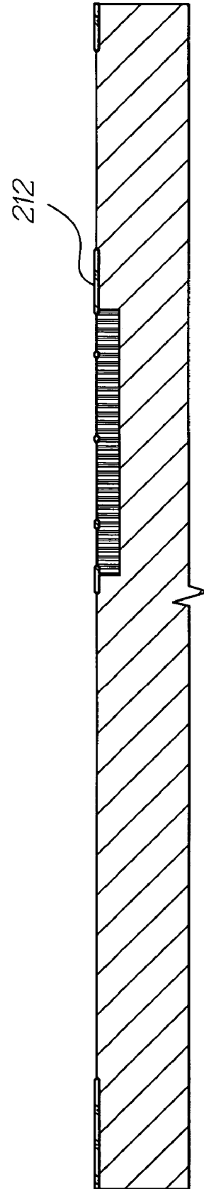
Grow field oxide
