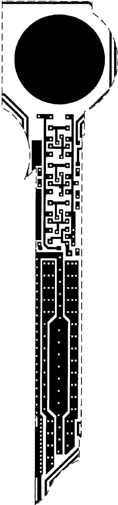
Metal 1 mask
