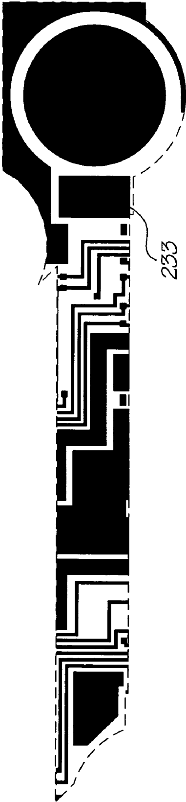
Metal 2 mask
