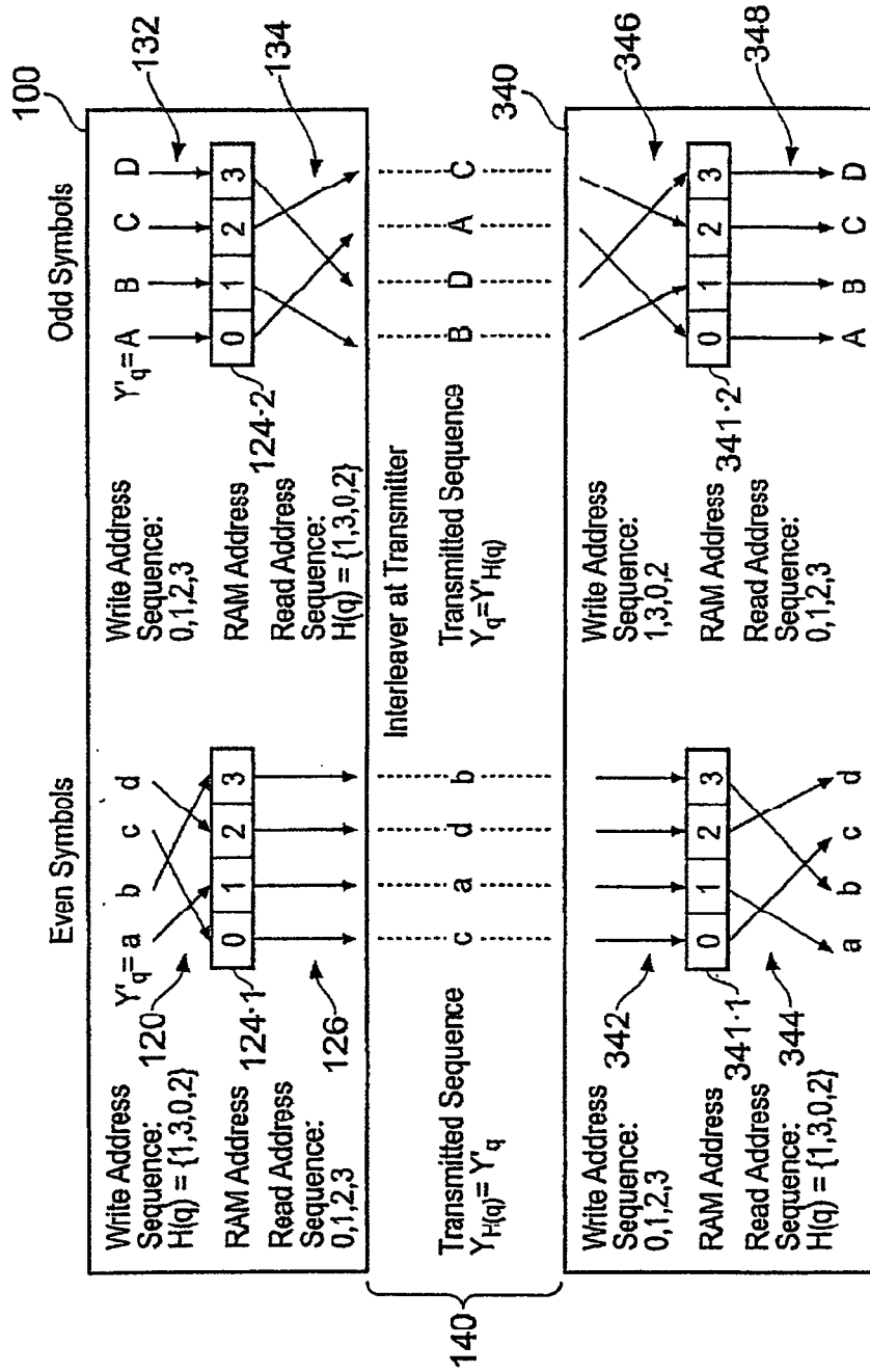
De-Interleaver at Receiver
