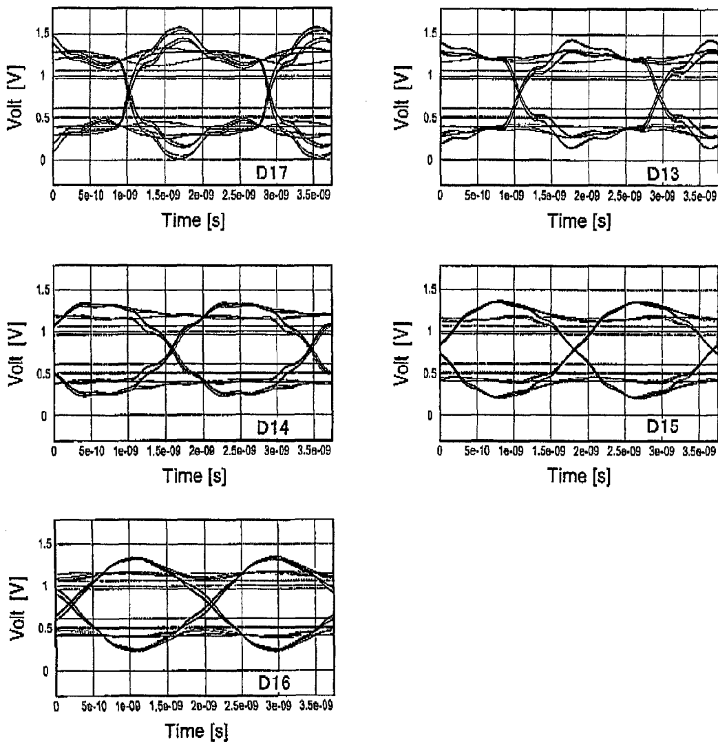
ADDRESS SIGNAL WAVEFORMS IN MEMORY ELEMENTS OF THIRD EMBODIMENT
