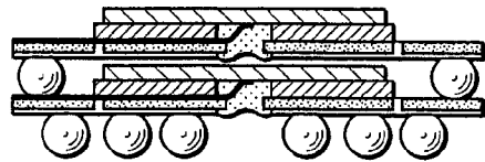
STACKED PACKAGE STRUCTURE
