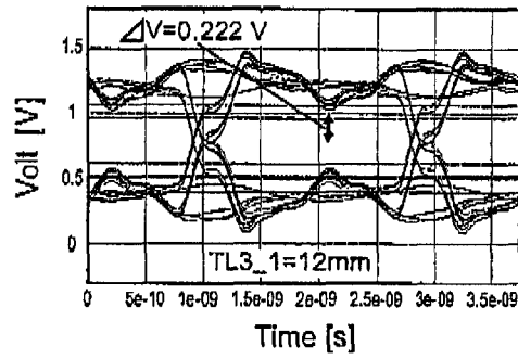
ADDRESS SIGNAL WAVEFORMS OF FIRST EMBODIMENT (D17)
