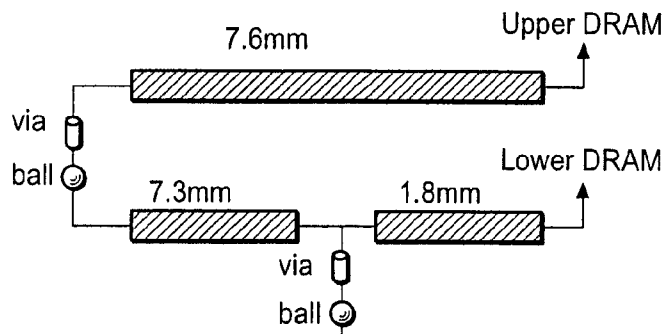
STACKED PACKAGE WIRING CONFIGURATION IN RELATED ART
