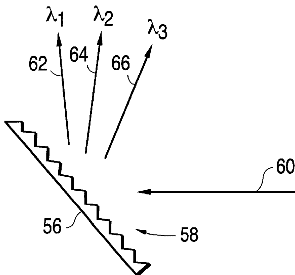
FIG. 5 (PRIOR ART)
