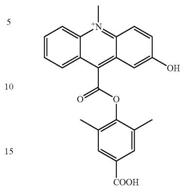
2-hydroxy-DMAE
