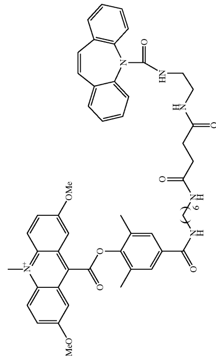
2,7-dimethoxy-DMAE-HD-SA-ED-Carbamazepine
