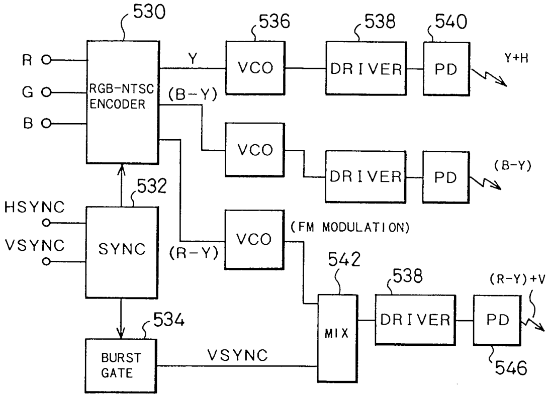
Fig. 15(a) MODULATOR UNIT IN CONTROL CIRCUIT UNIT
