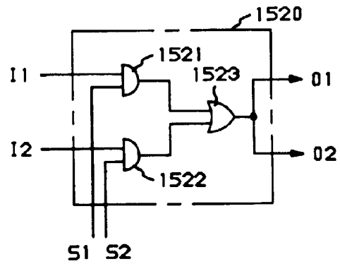
FIG. 7 CAPACITY ONE NODE WITH SELECTIVITY
