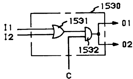
FIG. 8 CAPACITY ONE NODE WITHOUT SELECTIVITY
