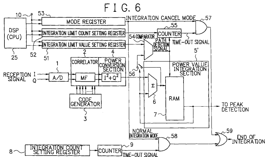
BLOCK DIAGRAM OF CELL SEARCH OF SECOND EMBODIMENT
