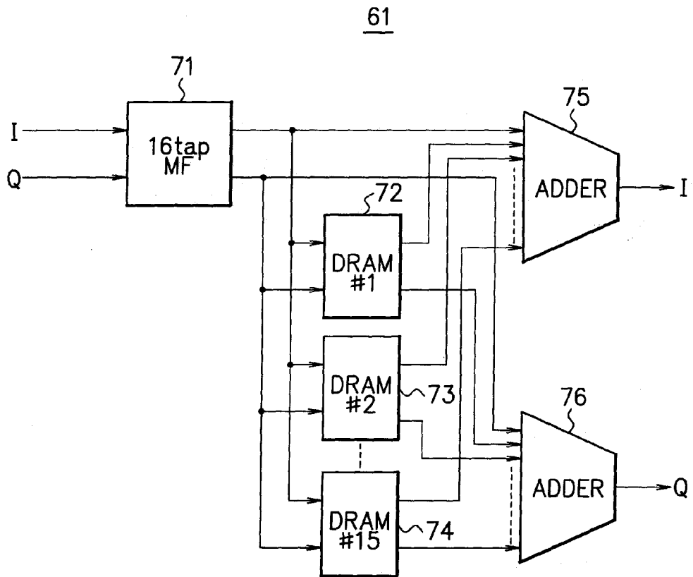
BLOCK DIAGRAM OF CORRELATOR OF THIRD EMBODIMENT
