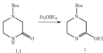
Scheme 1: General synthetic scheme for the preparation of the
