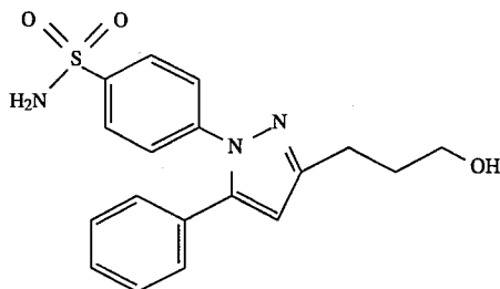
4-[5-Phenyl-3-(3-hydroxypropyl)-1H-pyrazol-1-yl]benzenesulfonamide
