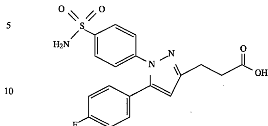
4-[4-(Aminosulfonyl)phenyl]-5-(4-fluorophenyl)-1H-pyrazole-3-propanoic acid
