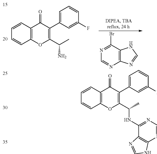
(S)-2-(1-(9H-purin-6-ylamino)ethyl)-6-bromo-3-phenyl-4H-chromen-4-one
