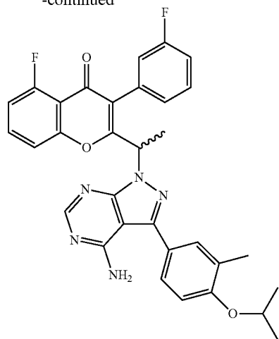
(-)-2-(1-(4-amino-3-(4-isopropoxy-3-methylphenyl)1H-pyrazolo[3,4-d]pyrimidin-4-yl)ethyl)-5-fluoro-3-(3-fluorophenyl)-4H-chromen-4-one
