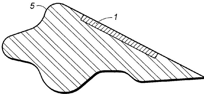
Fig. 2 (PRIOR ART)
