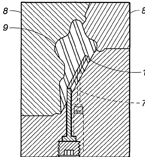
Fig. 5 (PRIOR ART)
