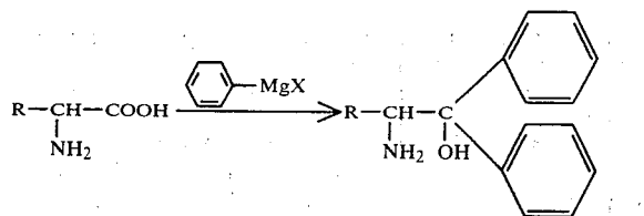
Reaction Scheme A
