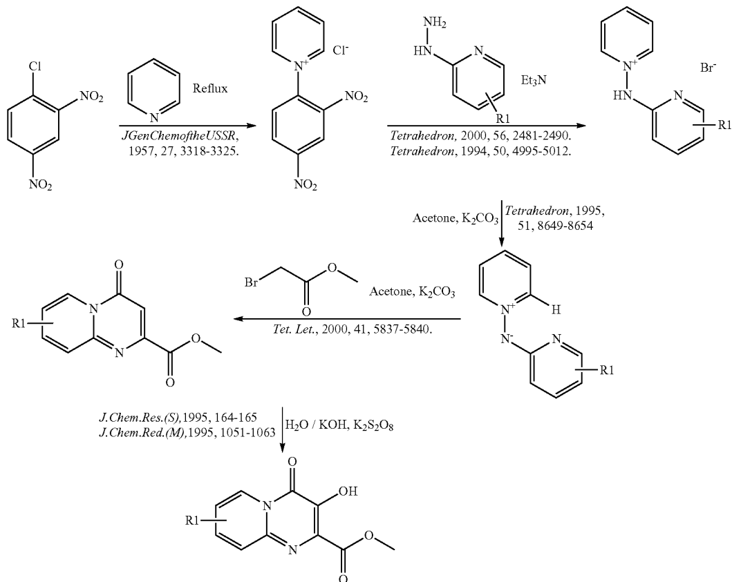
General Scheme 3: Alternate Synthesis 2
