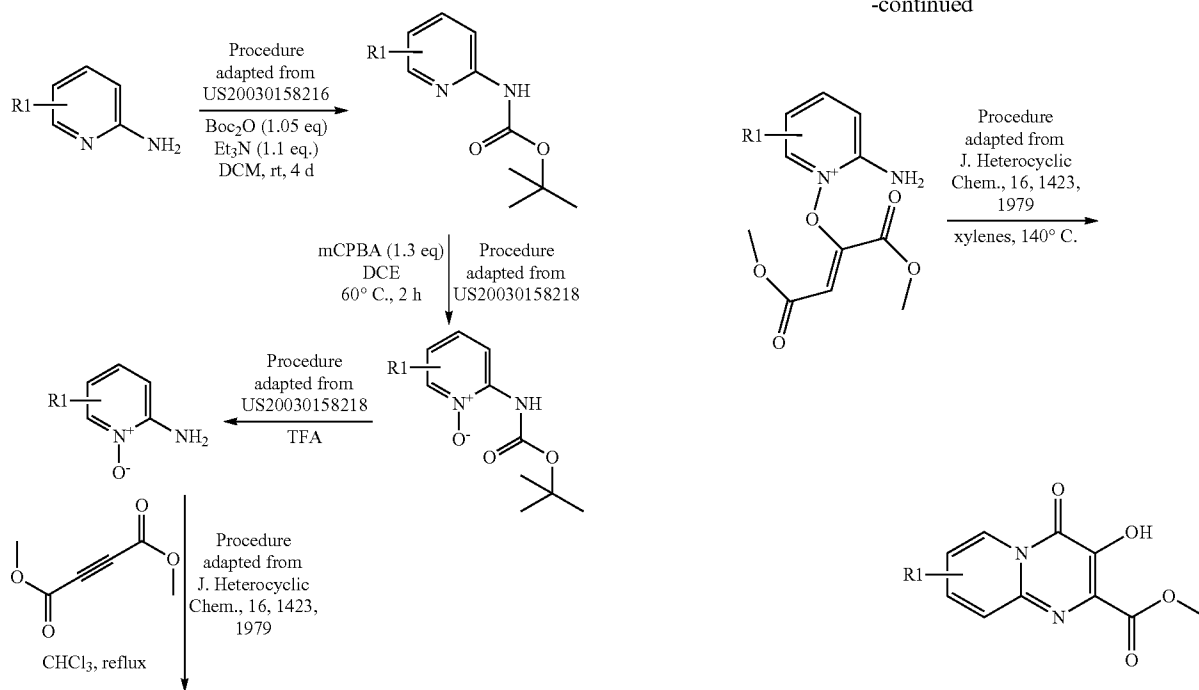
General Scheme 3: Alternate Synthesis 2
