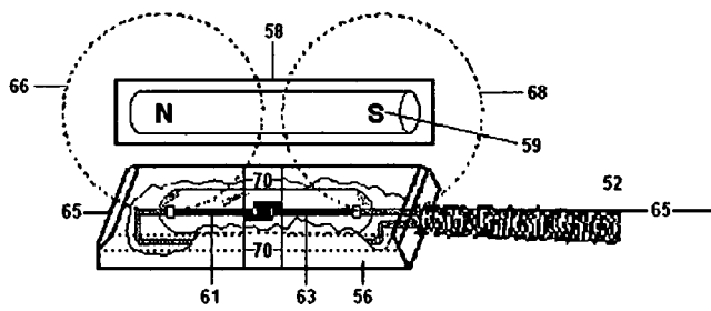
FIG 6B Normal Circuit PRIOR ART
