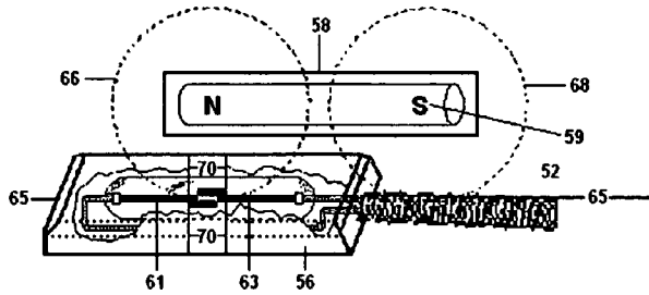
FIG 6D Faulted Circuit PRIOR ART
