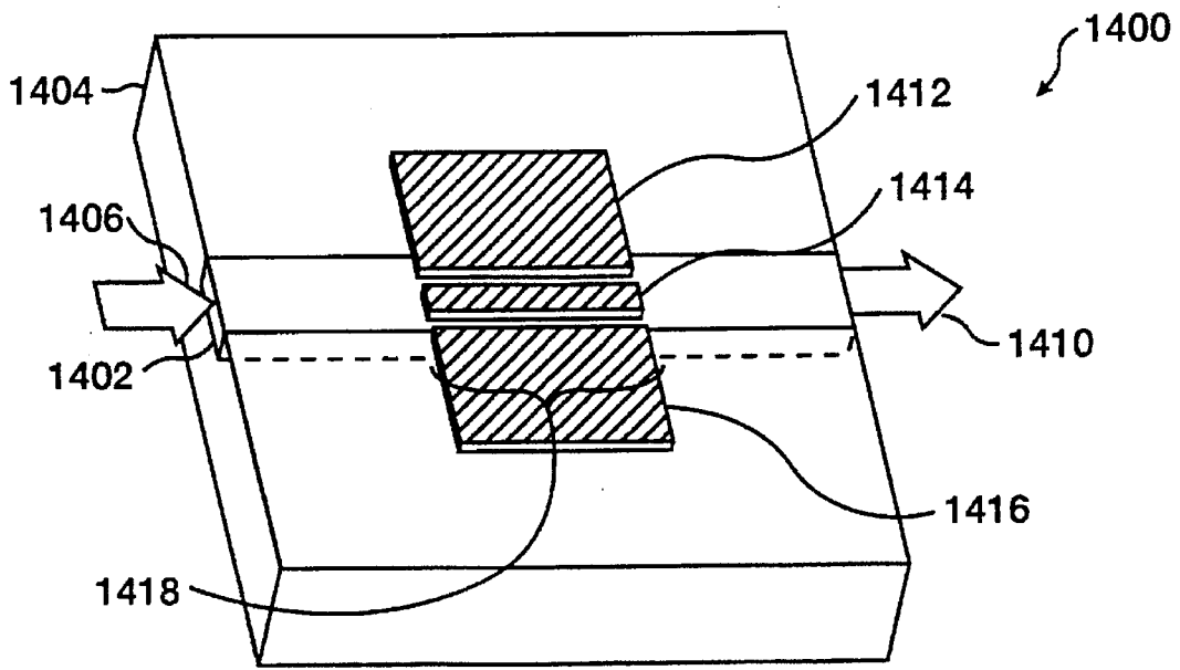
Figure 50 (Prior Art)
