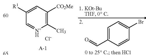
SCHEME A
