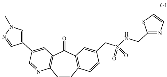
1-[3-(1-methyl-1H-pyrazol-4-yl)-5-oxo-5H-benzo[4,5]cyclohepta[1,2-b]pyridin-7-yl]-N-(1,3-thiazol-2-ylmethyl)methanesulfonamide (Compound 6-1)
