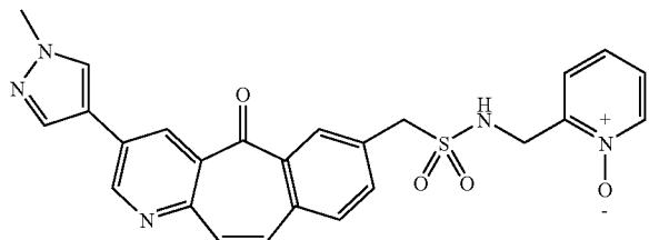
1-[3-(1-methyl-1H-pyrazol-4-yl)-5-oxo-5H-benzo[4,5]cyclohepta[1,2-b]pyridin-7-yl]-N-[(1-oxidopyridin-2-yl)methyl]methanesulfonamide (Compound 10-1)
