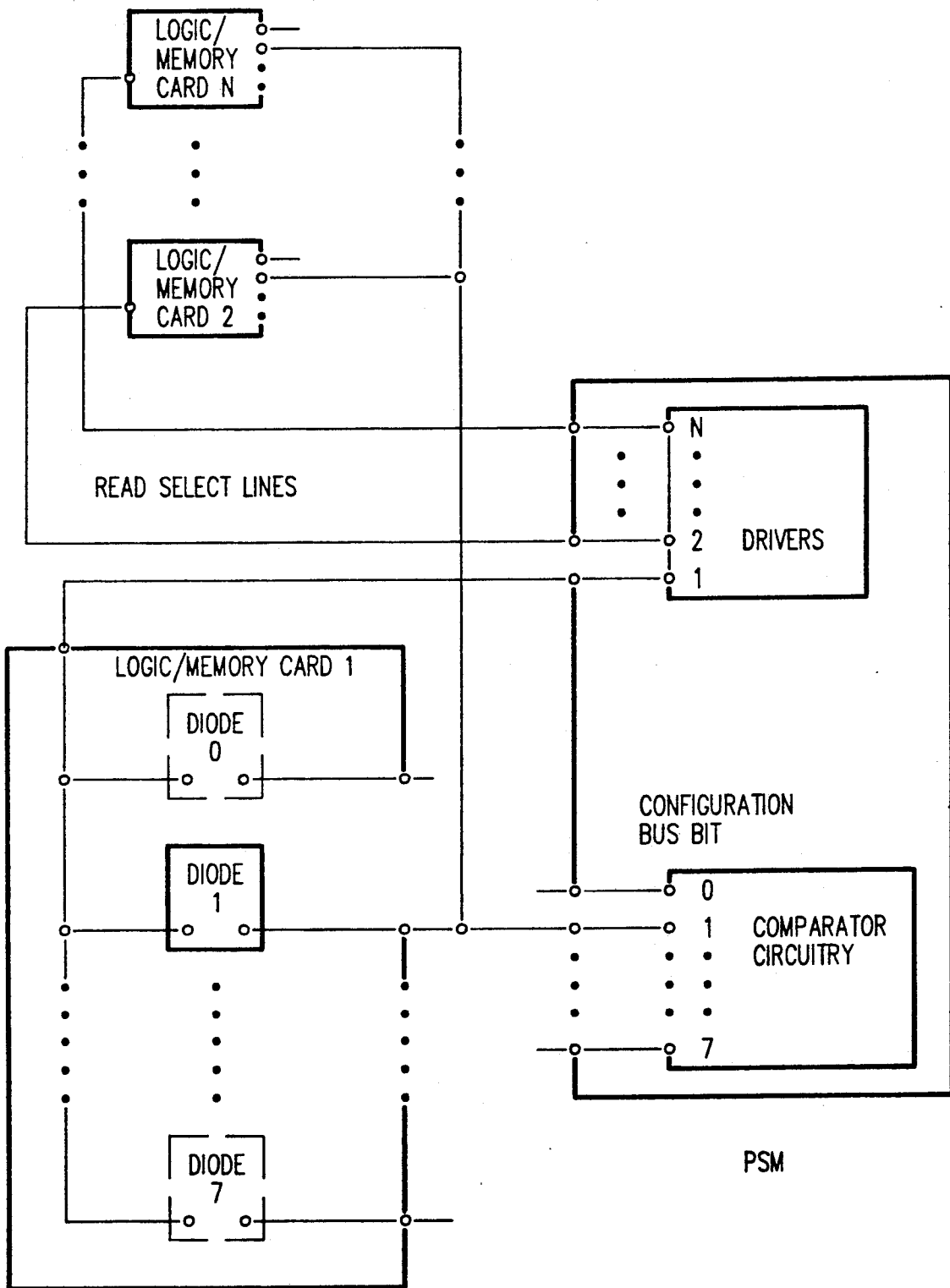
CONFIGURATION BUS STRUCTURE
